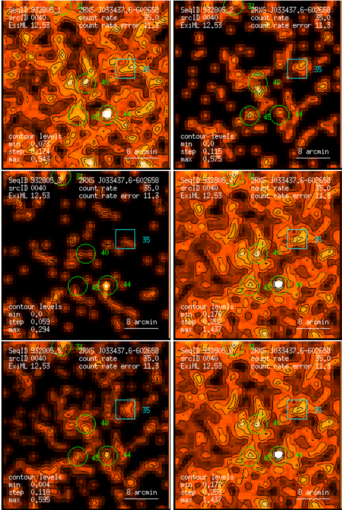
Figure 40: RASS 932805: detection 0040: band rate images, Gaussian filter: (1) PSPC channels 11 – 41, (2) 52 – 90, (3) 91 – 201, (4) 11 – 235, (5) 52 – 201, (6) 11 – 201. Broad band rates in counts/ks. Band rate contour levels in counts/ks/arcmin 2 .
