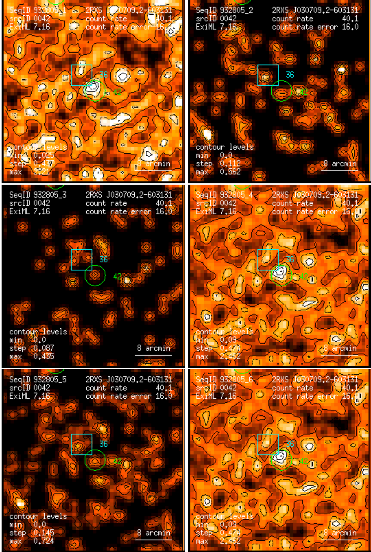
Figure 42: RASS 932805: detection 0042: band rate images, Gaussian filter: (1) PSPC channels 11 – 41, (2) 52 – 90, (3) 91 – 201, (4) 11 – 235, (5) 52 – 201, (6) 11 – 201. Broad band rates in counts/ks. Band rate contour levels in counts/ks/arcmin 2 .
