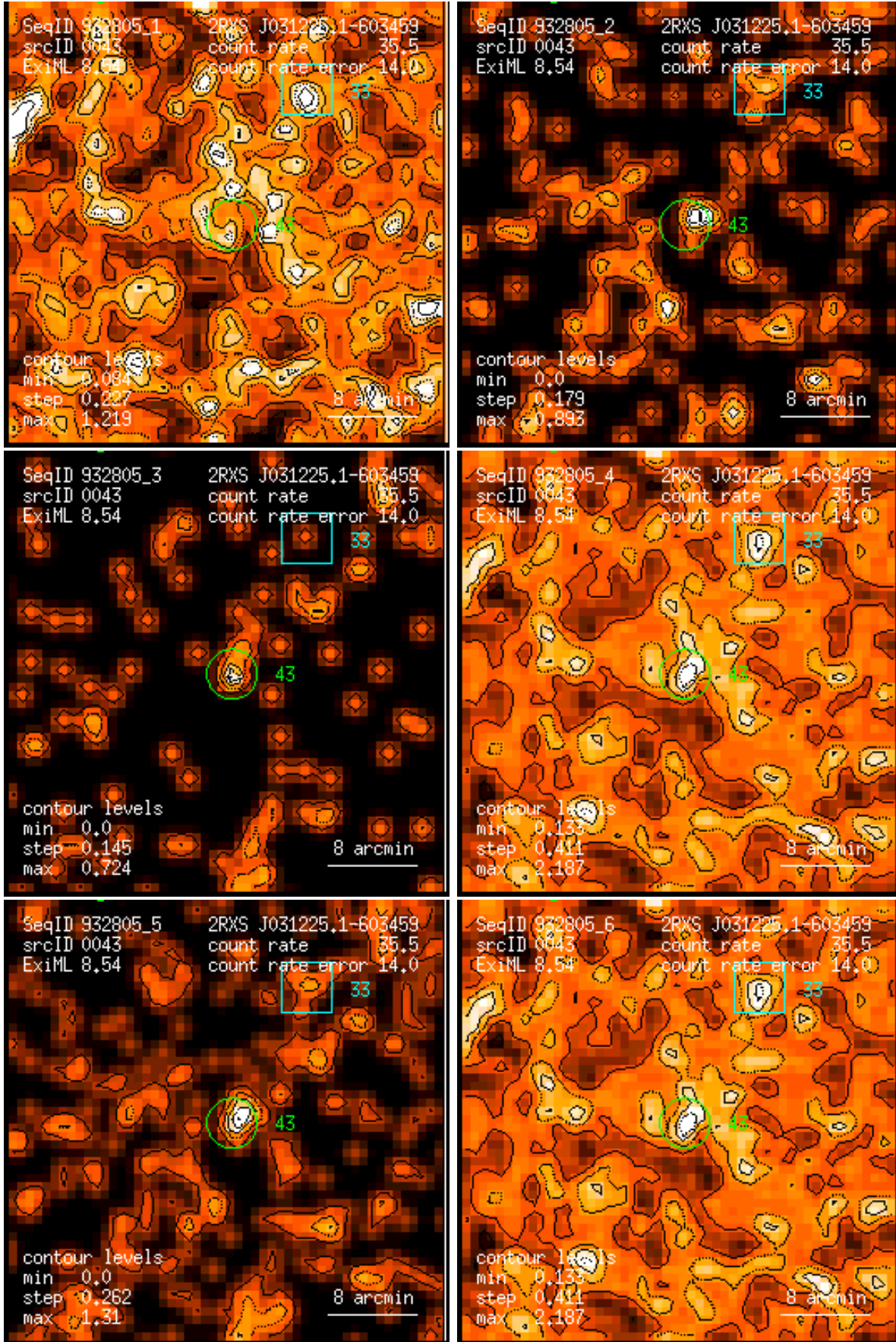
Figure 43: RASS 932805: detection 0043: band rate images, Gaussian filter: (1) PSPC channels 11 – 41, (2) 52 – 90, (3) 91 – 201, (4) 11 – 235, (5) 52 – 201, (6) 11 – 201. Broad band rates in counts/ks. Band rate contour levels in counts/ks/arcmin 2 .
