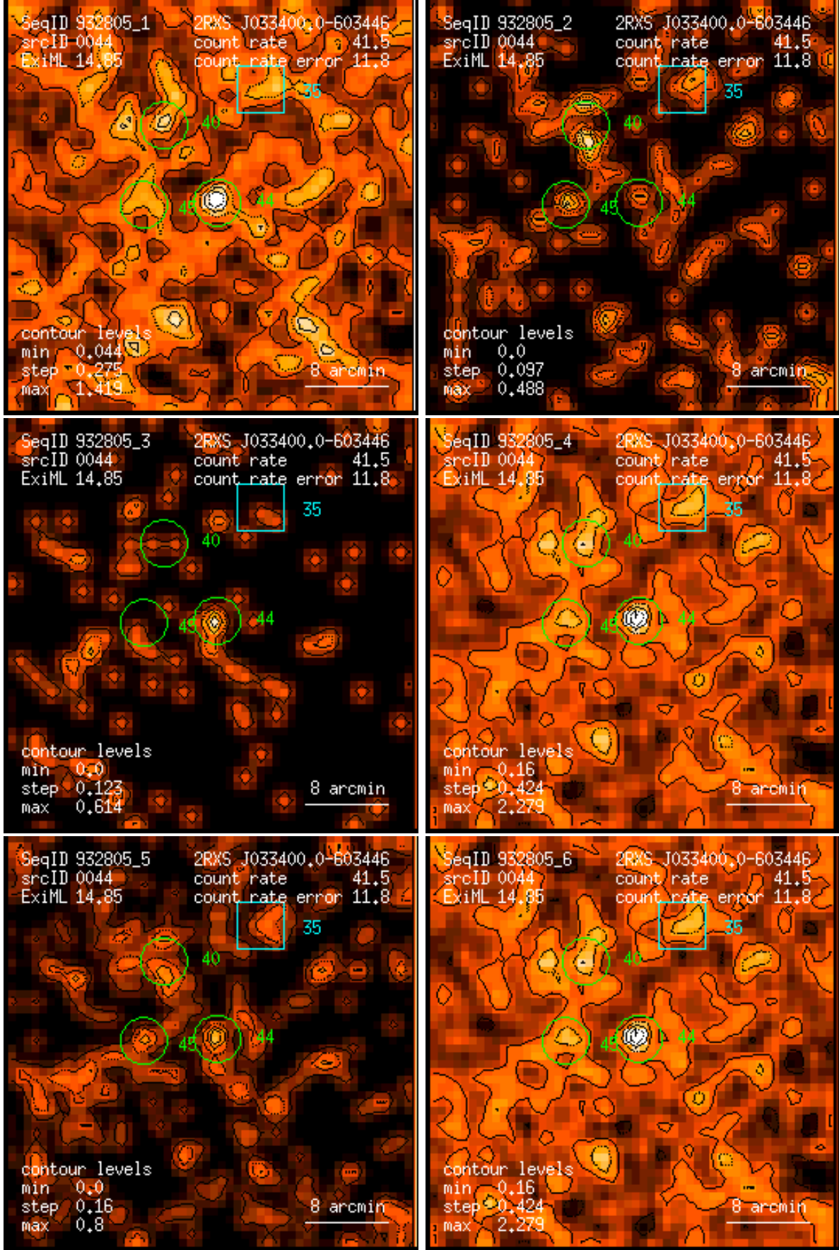
Figure 44: RASS 932805: detection 0044: band rate images, Gaussian filter: (1) PSPC channels 11 – 41, (2) 52 – 90, (3) 91 – 201, (4) 11 – 235, (5) 52 – 201, (6) 11 – 201. Broad band rates in counts/ks. Band rate contour levels in counts/ks/arcmin 2 .
