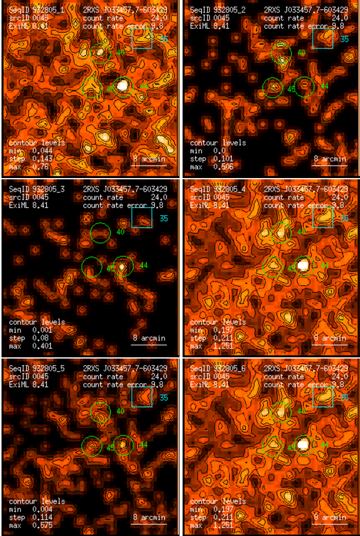
Figure 45: RASS 932805: detection 0045: band rate images, Gaussian filter: (1) PSPC channels 11 – 41, (2) 52 – 90, (3) 91 – 201, (4) 11 – 235, (5) 52 – 201, (6) 11 – 201. Broad band rates in counts/ks. Band rate contour levels in counts/ks/arcmin 2 .
