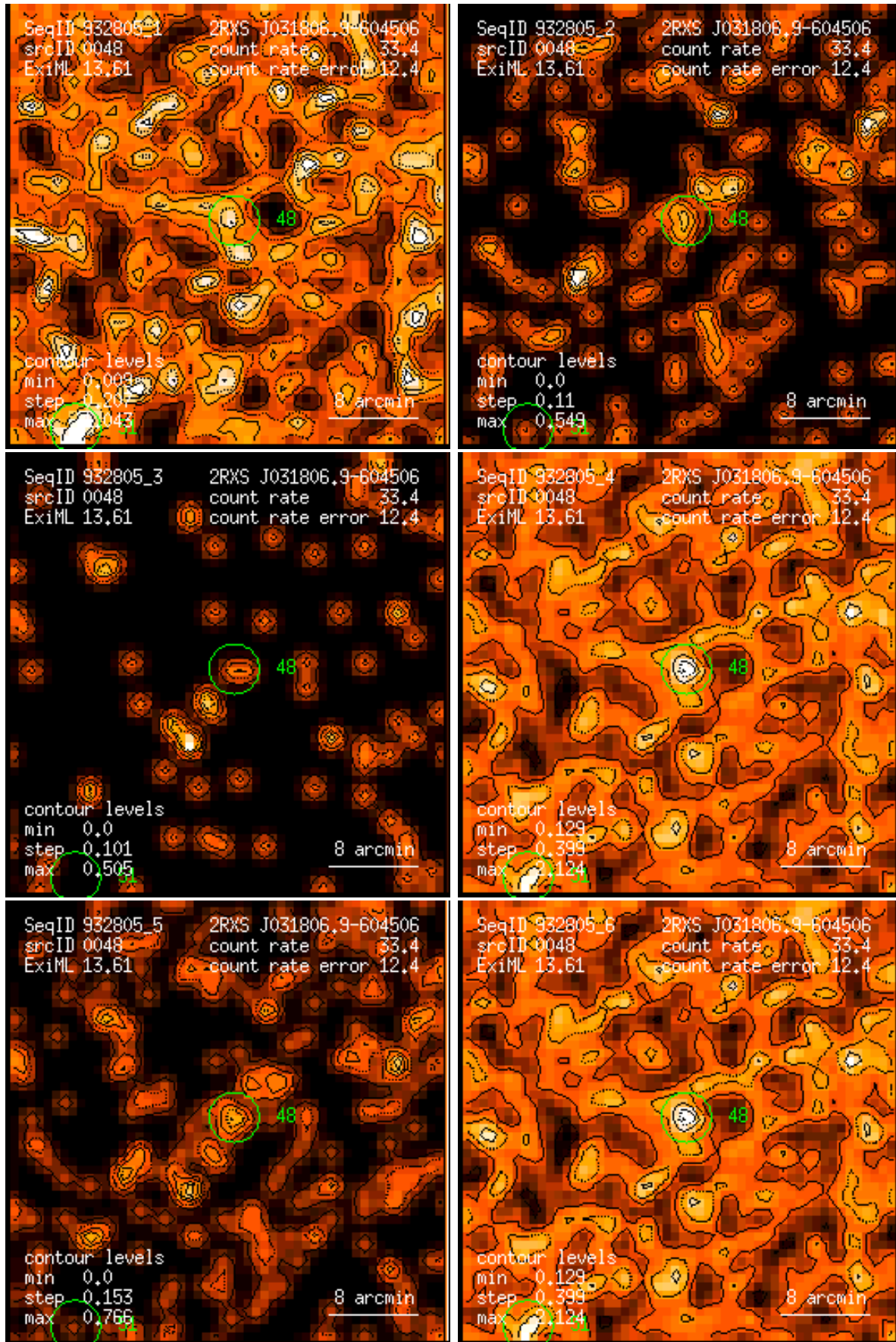
Figure 48: RASS 932805: detection 0048: band rate images, Gaussian filter: (1) PSPC channels 11 – 41, (2) 52 – 90, (3) 91 – 201, (4) 11 – 235, (5) 52 – 201, (6) 11 – 201. Broad band rates in counts/ks. Band rate contour levels in counts/ks/arcmin 2 .
