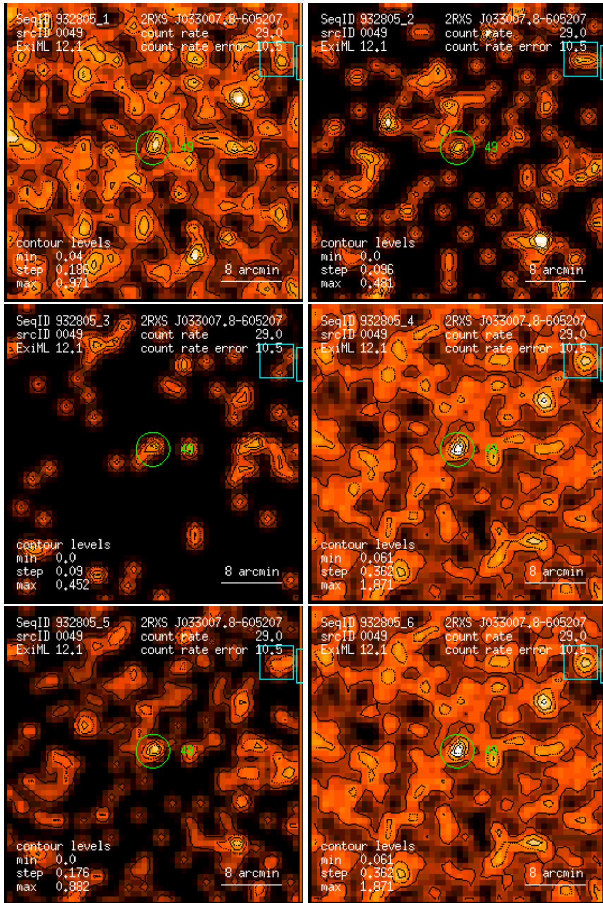
Figure 49: RASS 932805: detection 0049: band rate images, Gaussian filter: (1) PSPC channels 11 – 41, (2) 52 – 90, (3) 91 – 201, (4) 11 – 235, (5) 52 – 201, (6) 11 – 201. Broad band rates in counts/ks. Band rate contour levels in counts/ks/arcmin 2 .
