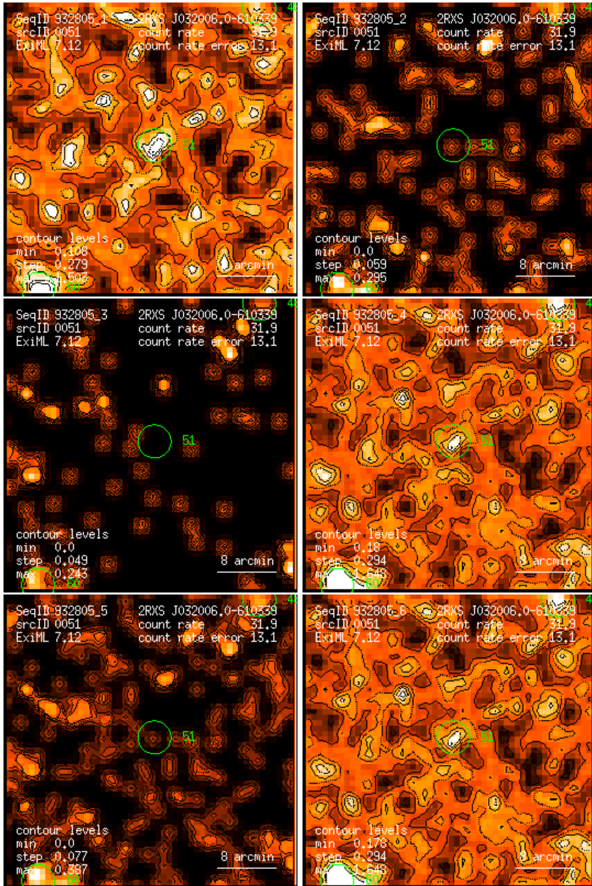
Figure 51: RASS 932805: detection 0051: band rate images, Gaussian filter: (1) PSPC channels 11 – 41, (2) 52 – 90, (3) 91 – 201, (4) 11 – 235, (5) 52 – 201, (6) 11 – 201. Broad band rates in counts/ks. Band rate contour levels in counts/ks/arcmin 2 .
