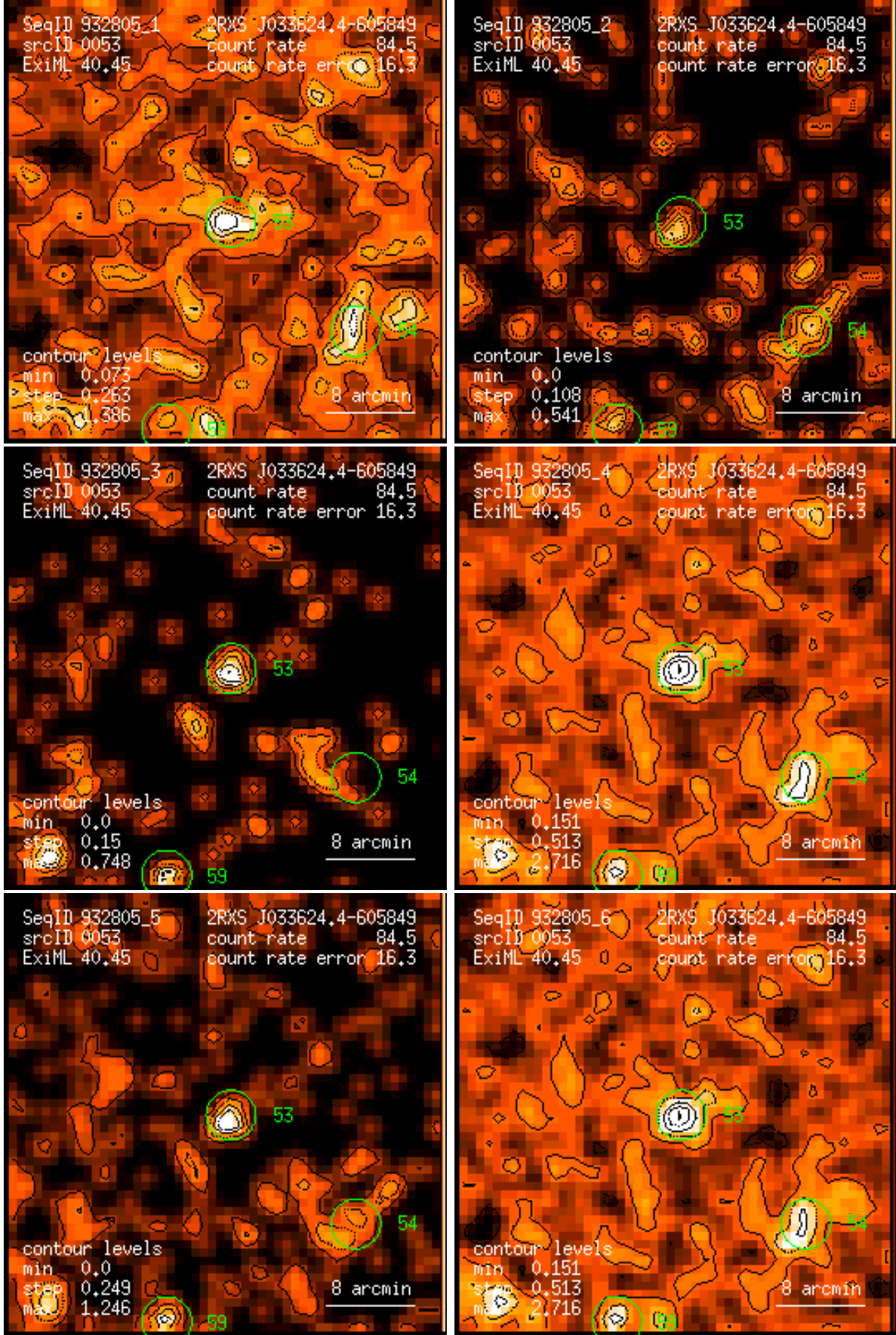
Figure 53: RASS 932805: detection 0053: band rate images, Gaussian filter: (1) PSPC channels 11 – 41, (2) 52 – 90, (3) 91 – 201, (4) 11 – 235, (5) 52 – 201, (6) 11 – 201. Broad band rates in counts/ks. Band rate contour levels in counts/ks/arcmin 2 .
