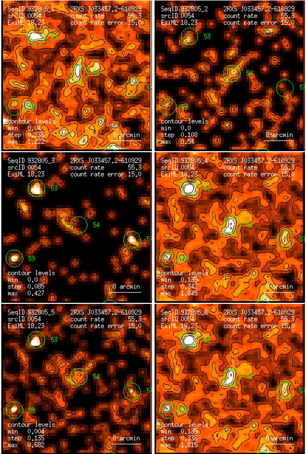
Figure 54: RASS 932805: detection 0054: band rate images, Gaussian filter: (1) PSPC channels 11 – 41, (2) 52 – 90, (3) 91 – 201, (4) 11 – 235, (5) 52 – 201, (6) 11 – 201. Broad band rates in counts/ks. Band rate contour levels in counts/ks/arcmin 2 .
