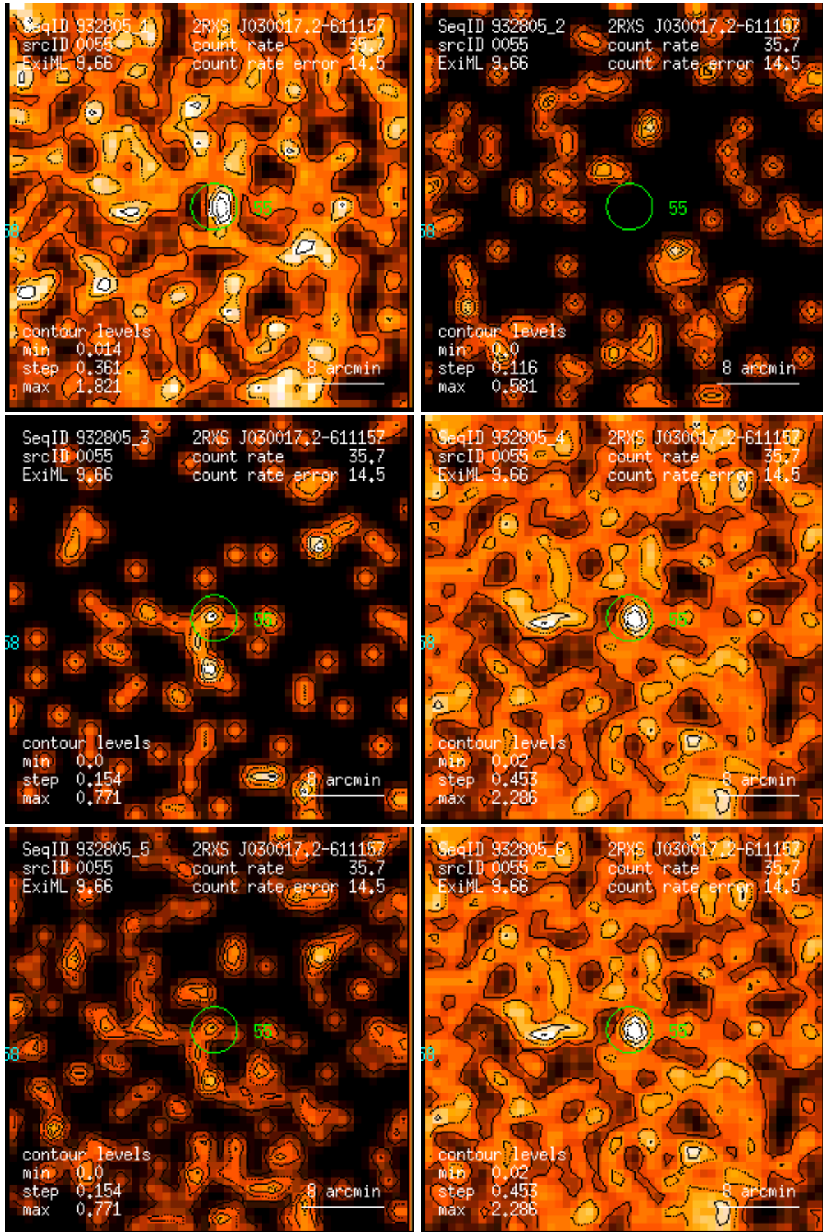
Figure 55: RASS 932805: detection 0055: band rate images, Gaussian filter: (1) PSPC channels 11 – 41, (2) 52 – 90, (3) 91 – 201, (4) 11 – 235, (5) 52 – 201, (6) 11 – 201. Broad band rates in counts/ks. Band rate contour levels in counts/ks/arcmin 2 .
