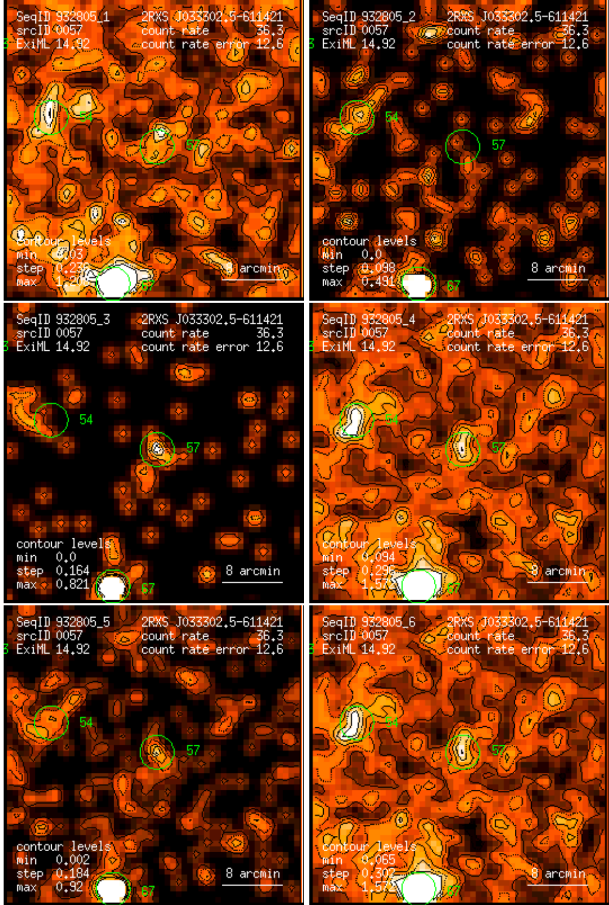
Figure 57: RASS 932805: detection 0057: band rate images, Gaussian filter: (1) PSPC channels 11 – 41, (2) 52 – 90, (3) 91 – 201, (4) 11 – 235, (5) 52 – 201, (6) 11 – 201. Broad band rates in counts/ks. Band rate contour levels in counts/ks/arcmin 2 .
