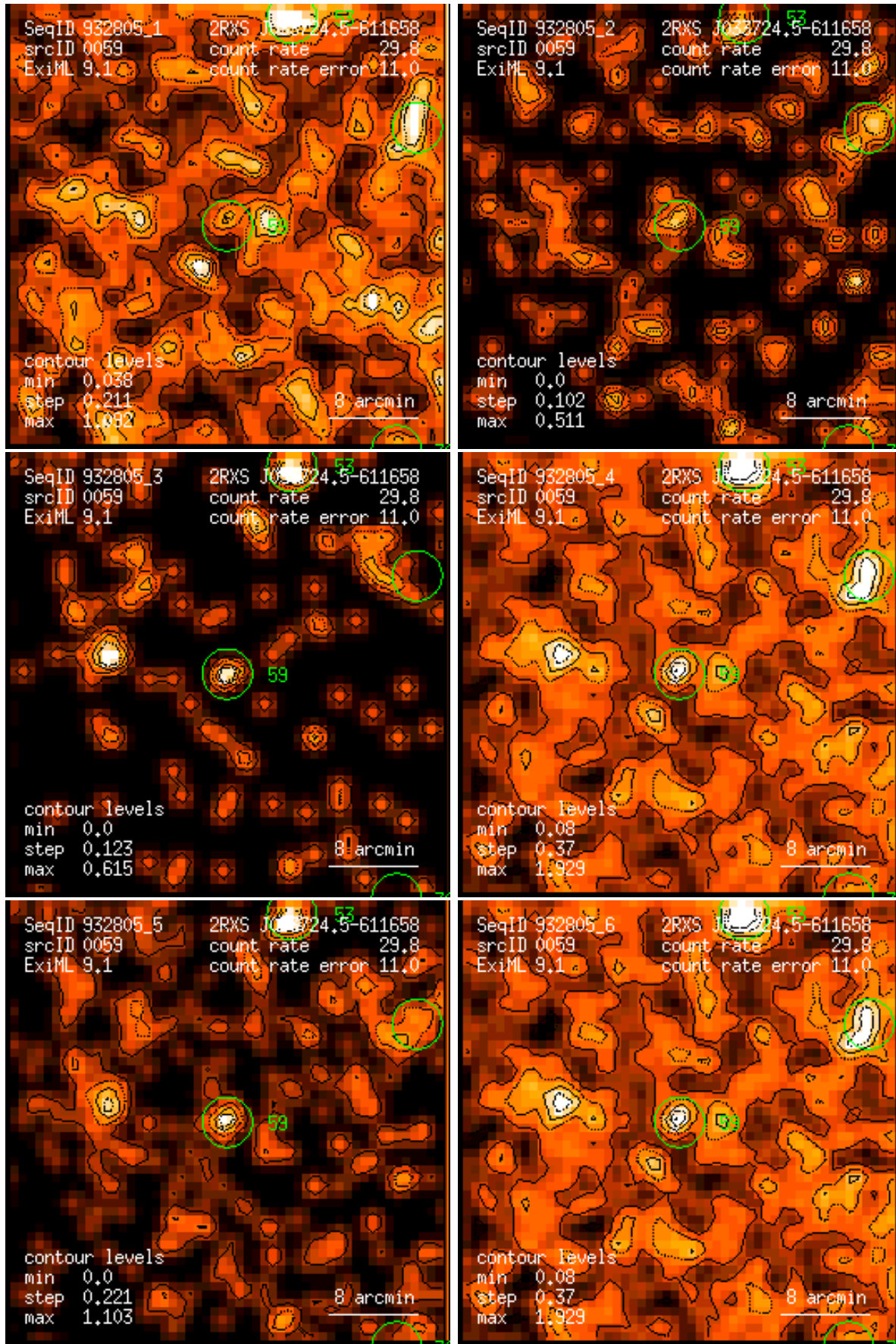
Figure 59: RASS 932805: detection 0059: band rate images, Gaussian filter: (1) PSPC channels 11 – 41, (2) 52 – 90, (3) 91 – 201, (4) 11 – 235, (5) 52 – 201, (6) 11 – 201. Broad band rates in counts/ks. Band rate contour levels in counts/ks/arcmin 2 .
