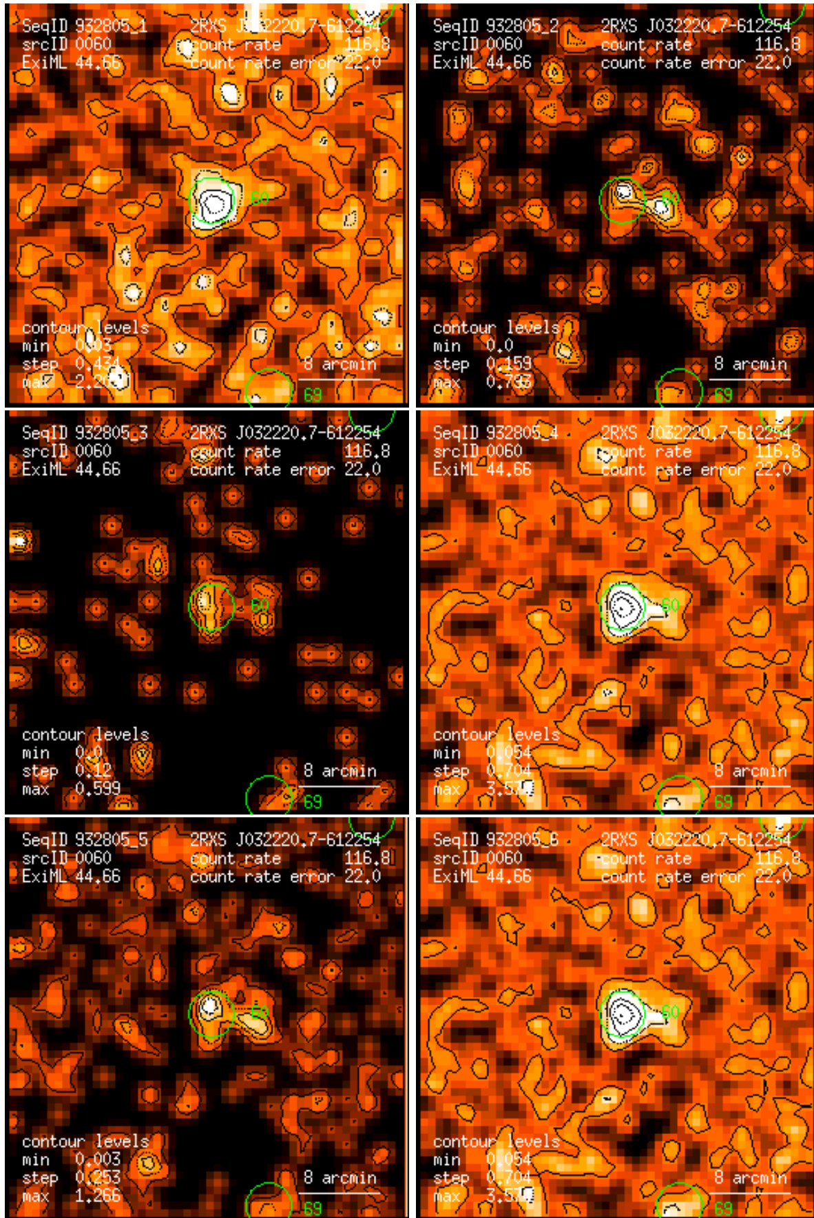
Figure 60: RASS 932805: detection 0060: band rate images, Gaussian filter: (1) PSPC channels 11 – 41, (2) 52 – 90, (3) 91 – 201, (4) 11 – 235, (5) 52 – 201, (6) 11 – 201. Broad band rates in counts/ks. Band rate contour levels in counts/ks/arcmin 2 .
