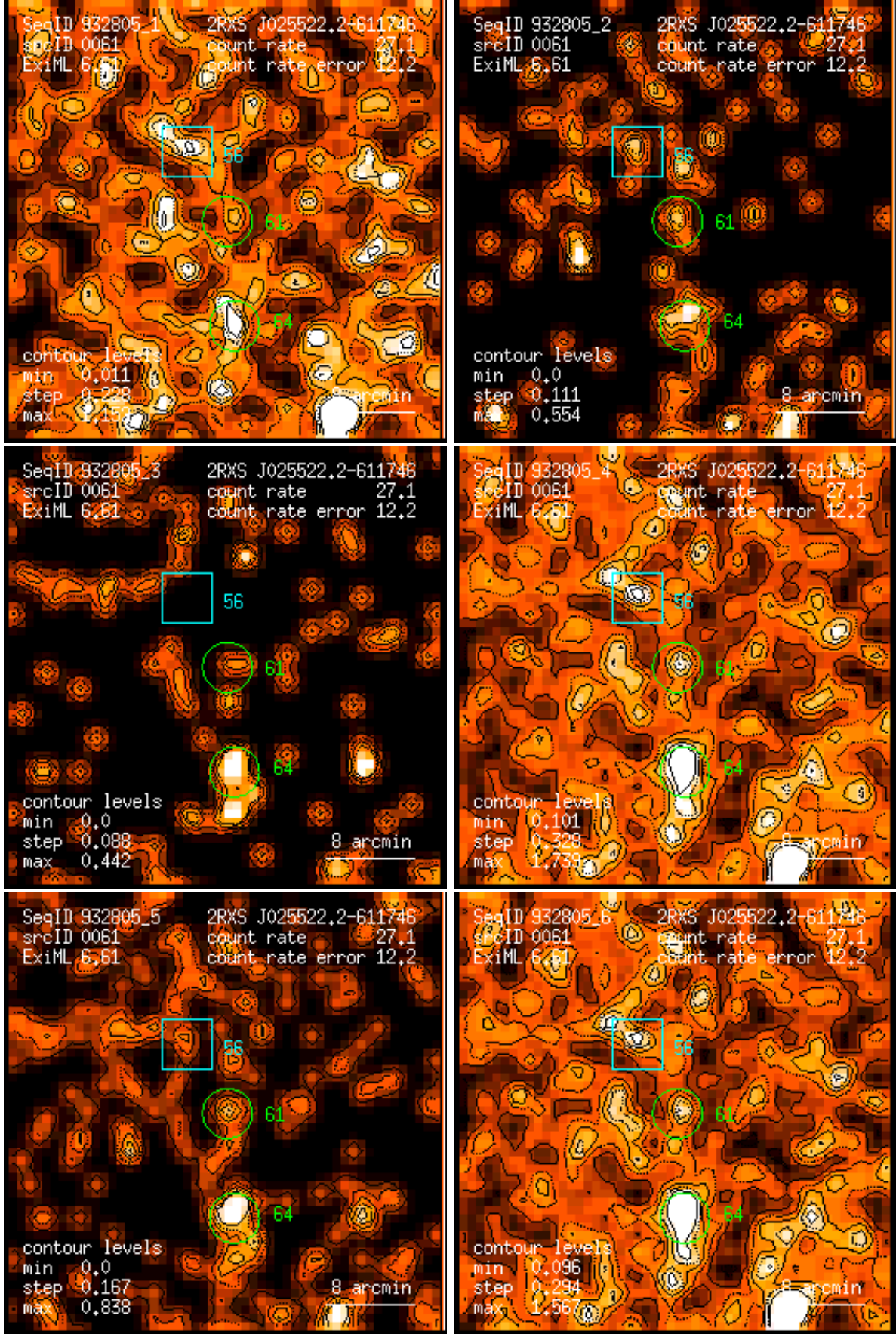
Figure 61: RASS 932805: detection 0061: band rate images, Gaussian filter: (1) PSPC channels 11 – 41, (2) 52 – 90, (3) 91 – 201, (4) 11 – 235, (5) 52 – 201, (6) 11 – 201. Broad band rates in counts/ks. Band rate contour levels in counts/ks/arcmin 2 .
