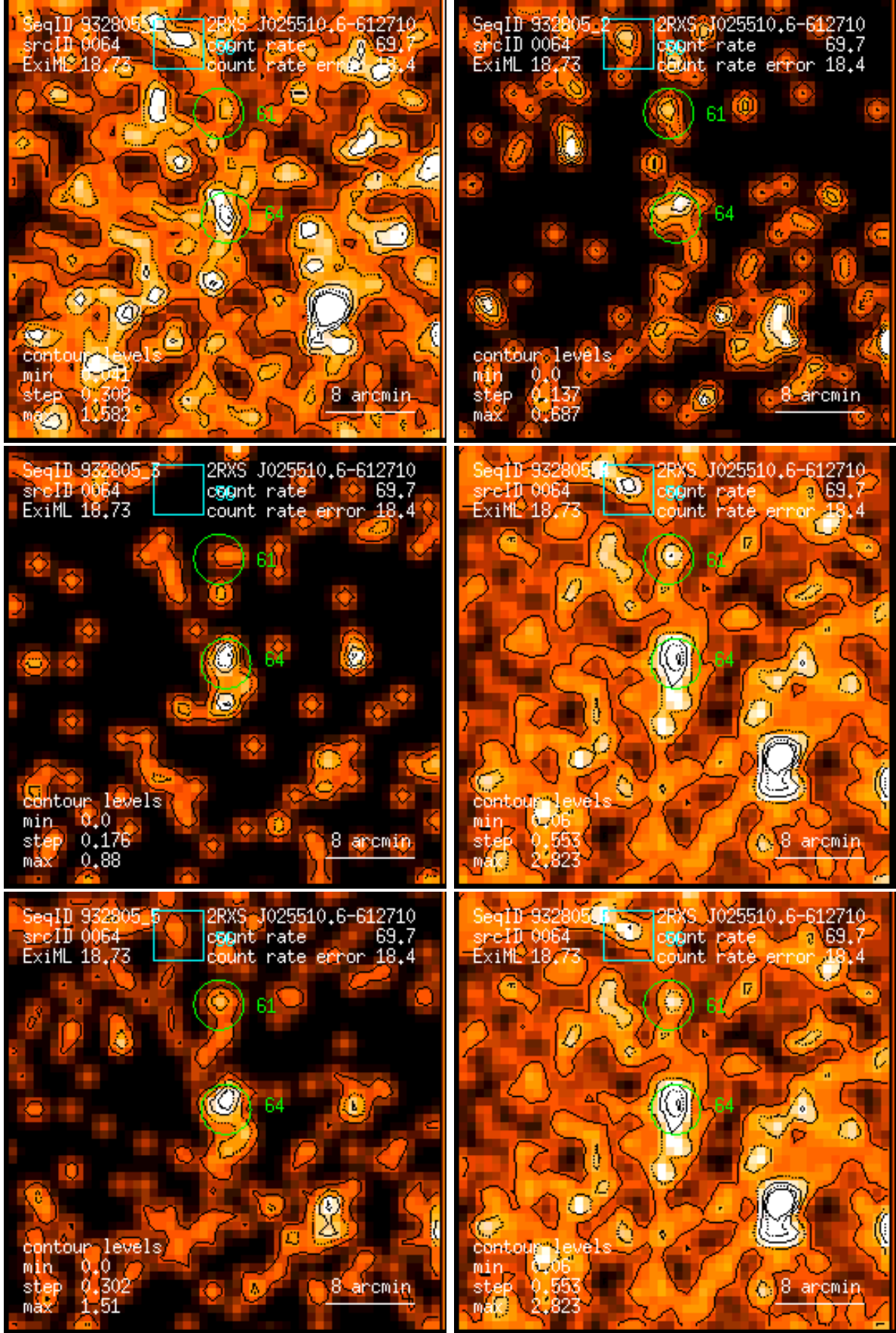
Figure 64: RASS 932805: detection 0064: band rate images, Gaussian filter: (1) PSPC channels 11 – 41, (2) 52 – 90, (3) 91 – 201, (4) 11 – 235, (5) 52 – 201, (6) 11 – 201. Broad band rates in counts/ks. Band rate contour levels in counts/ks/arcmin 2 .
