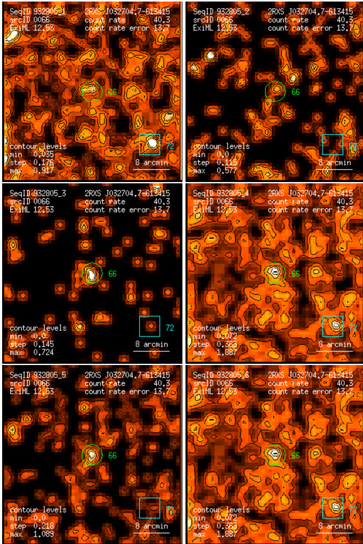
Figure 66: RASS 932805: detection 0066: band rate images, Gaussian filter: (1) PSPC channels 11 – 41, (2) 52 – 90, (3) 91 – 201, (4) 11 – 235, (5) 52 – 201, (6) 11 – 201. Broad band rates in counts/ks. Band rate contour levels in counts/ks/arcmin 2 .
