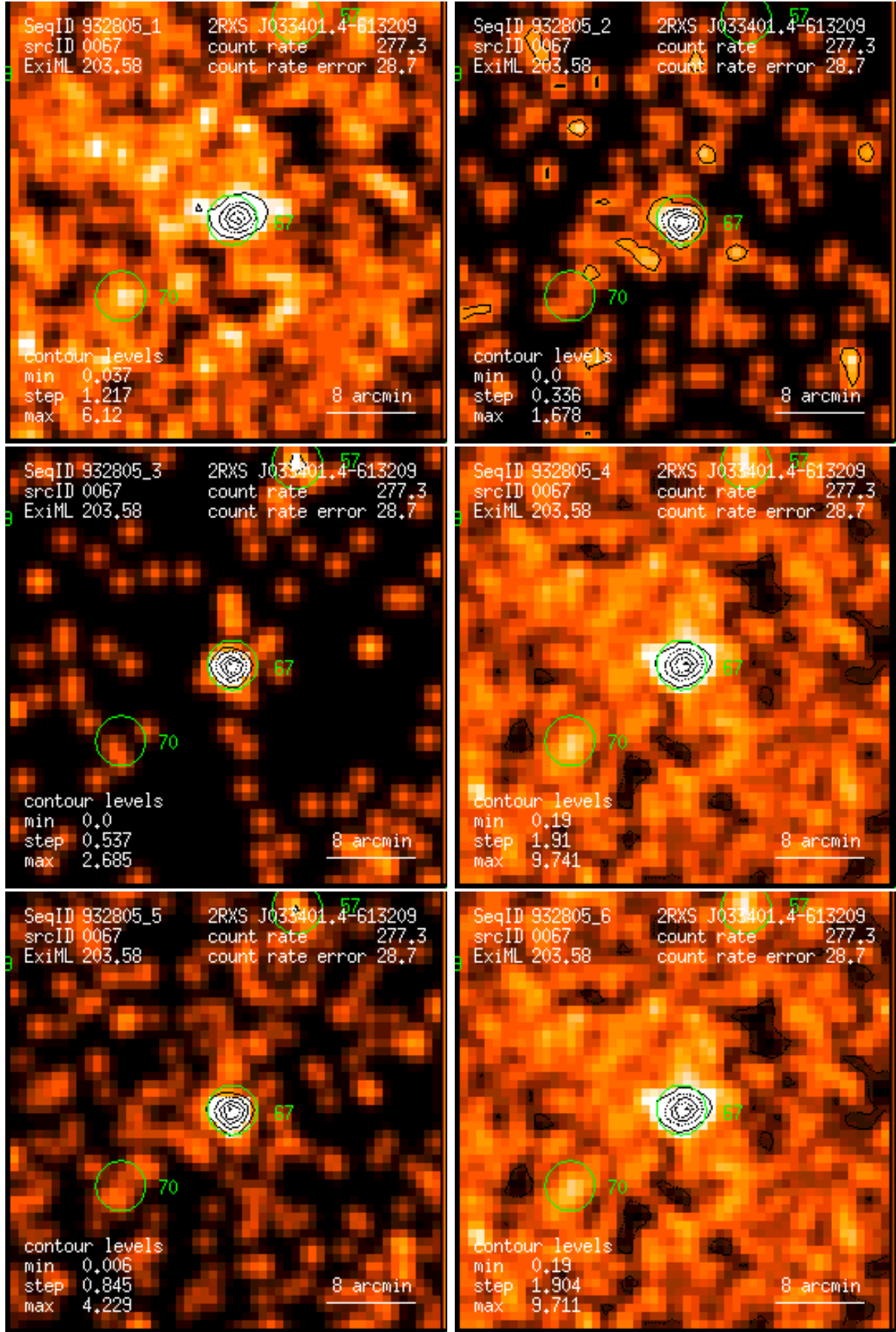
Figure 67: RASS 932805: detection 0067: band rate images, Gaussian filter: (1) PSPC channels 11 – 41, (2) 52 – 90, (3) 91 – 201, (4) 11 – 235, (5) 52 – 201, (6) 11 – 201. Broad band rates in counts/ks. Band rate contour levels in counts/ks/arcmin 2 .
