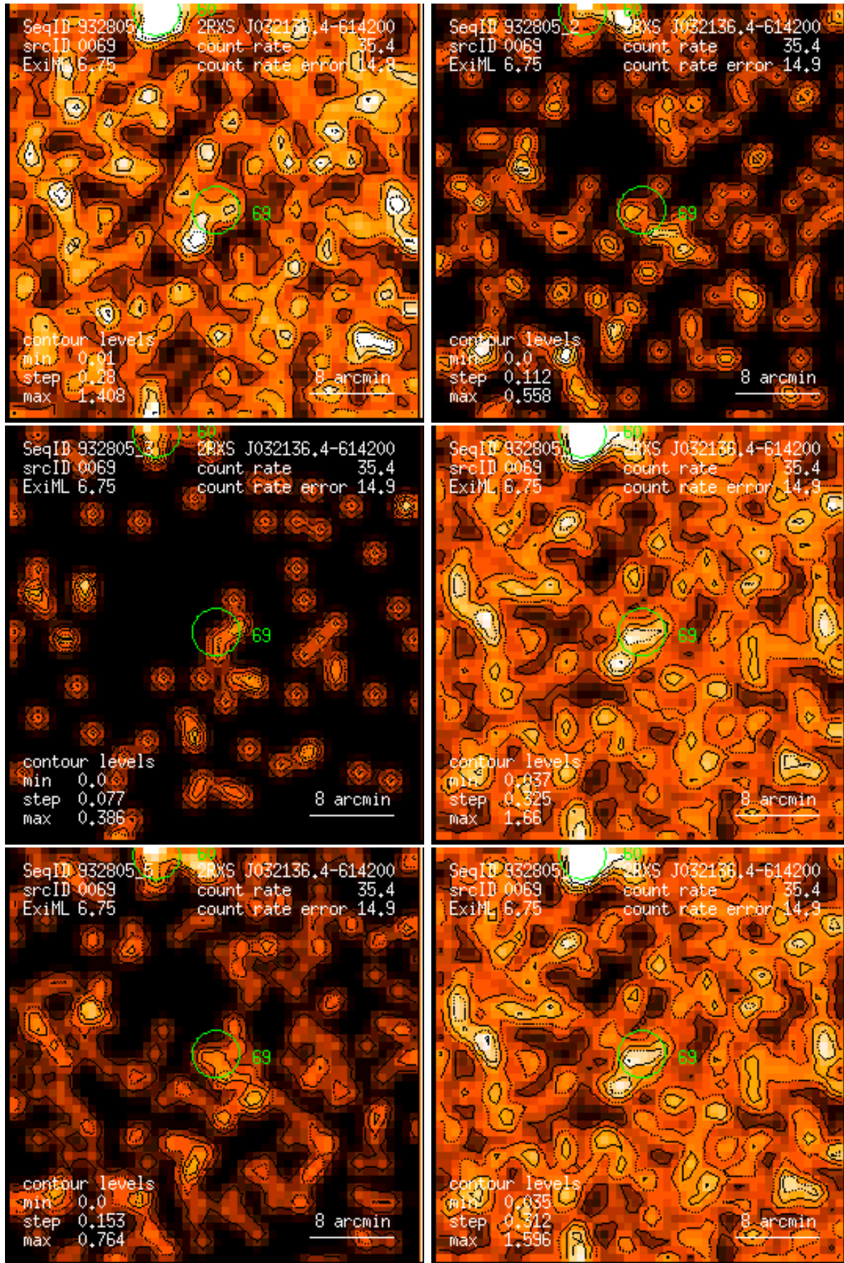
Figure 69: RASS 932805: detection 0069: band rate images, Gaussian filter: (1) PSPC channels 11 – 41, (2) 52 – 90, (3) 91 – 201, (4) 11 – 235, (5) 52 – 201, (6) 11 – 201. Broad band rates in counts/ks. Band rate contour levels in counts/ks/arcmin 2 .
