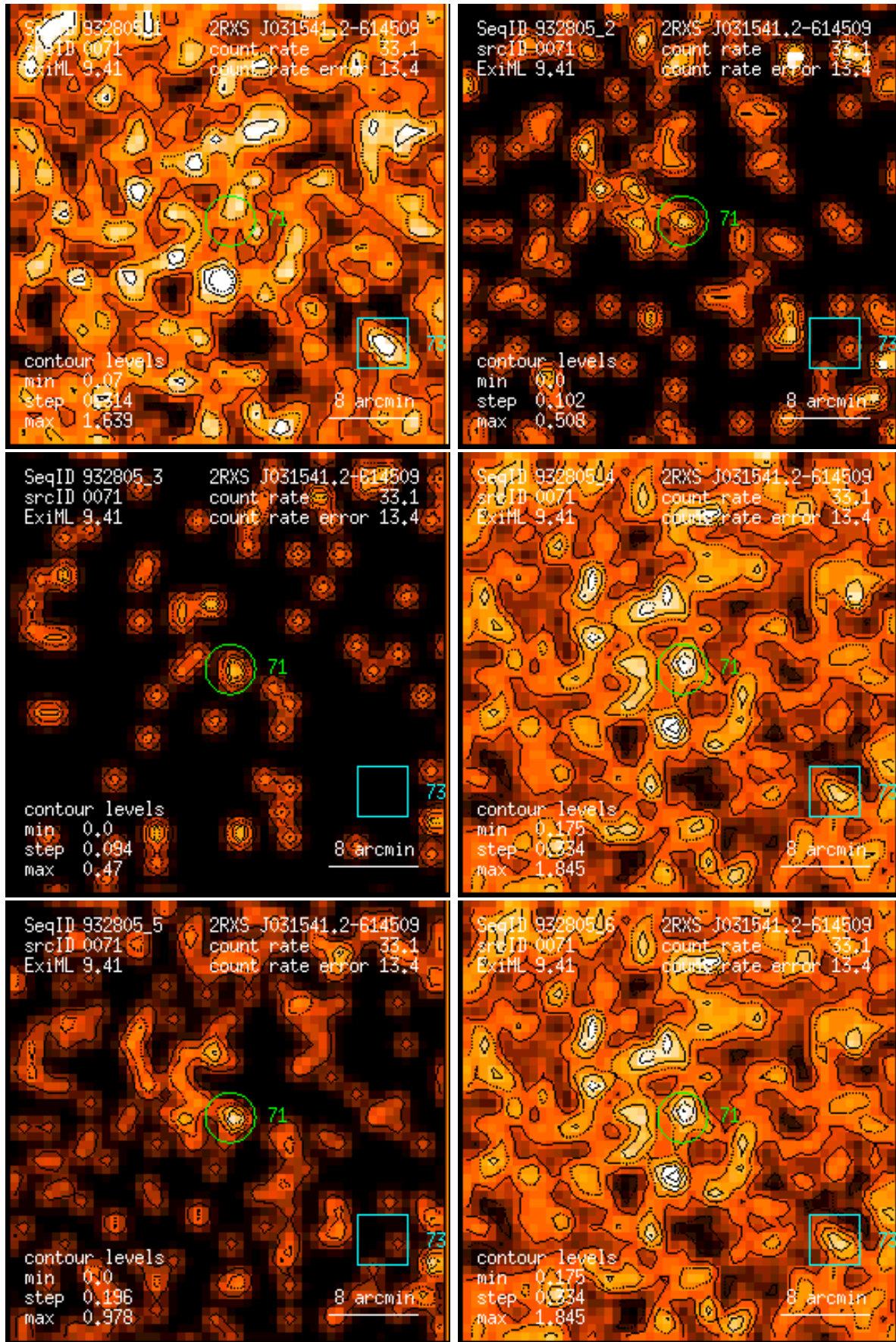
Figure 71: RASS 932805: detection 0071: band rate images, Gaussian filter: (1) PSPC channels 11 – 41, (2) 52 – 90, (3) 91 – 201, (4) 11 – 235, (5) 52 – 201, (6) 11 – 201. Broad band rates in counts/ks. Band rate contour levels in counts/ks/arcmin 2 .
