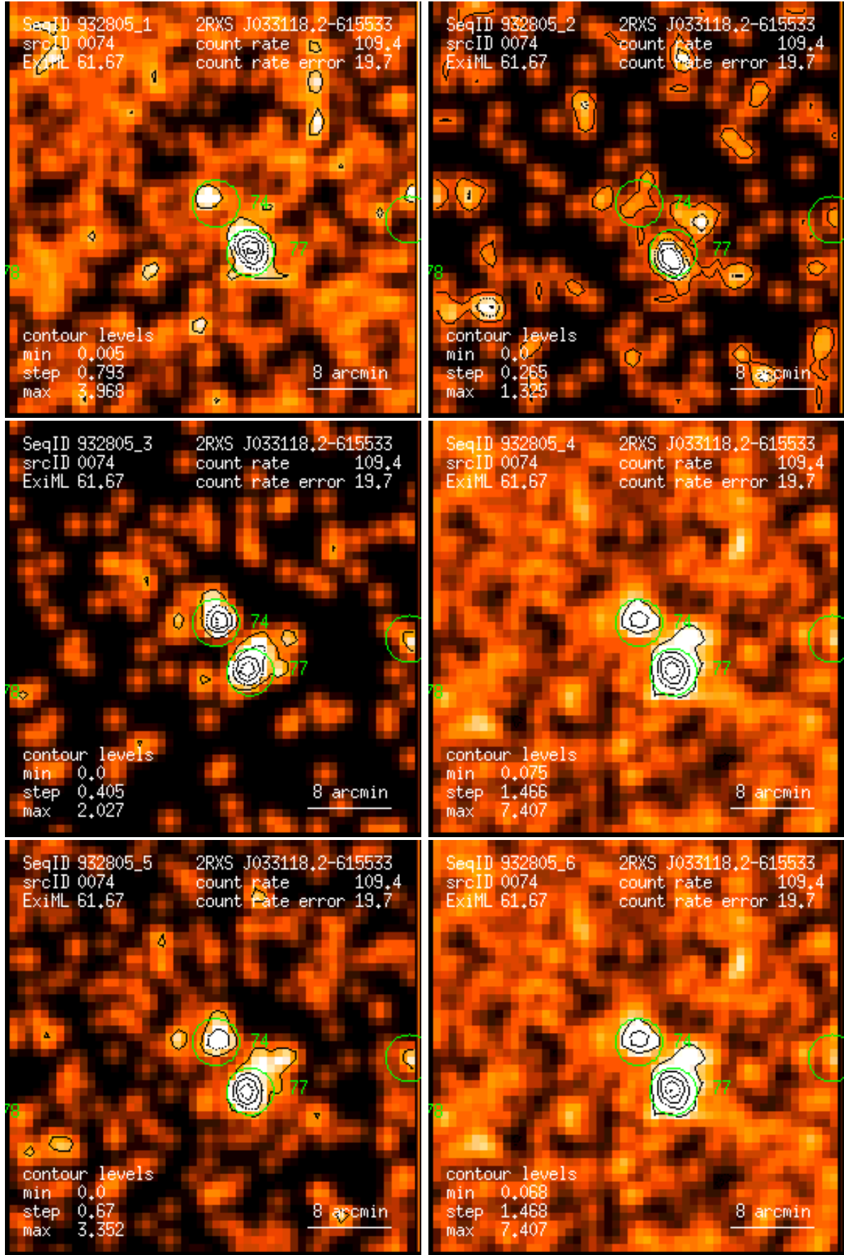
Figure 74: RASS 932805: detection 0074: band rate images, Gaussian filter: (1) PSPC channels 11 – 41, (2) 52 – 90, (3) 91 – 201, (4) 11 – 235, (5) 52 – 201, (6) 11 – 201. Broad band rates in counts/ks. Band rate contour levels in counts/ks/arcmin 2 .
