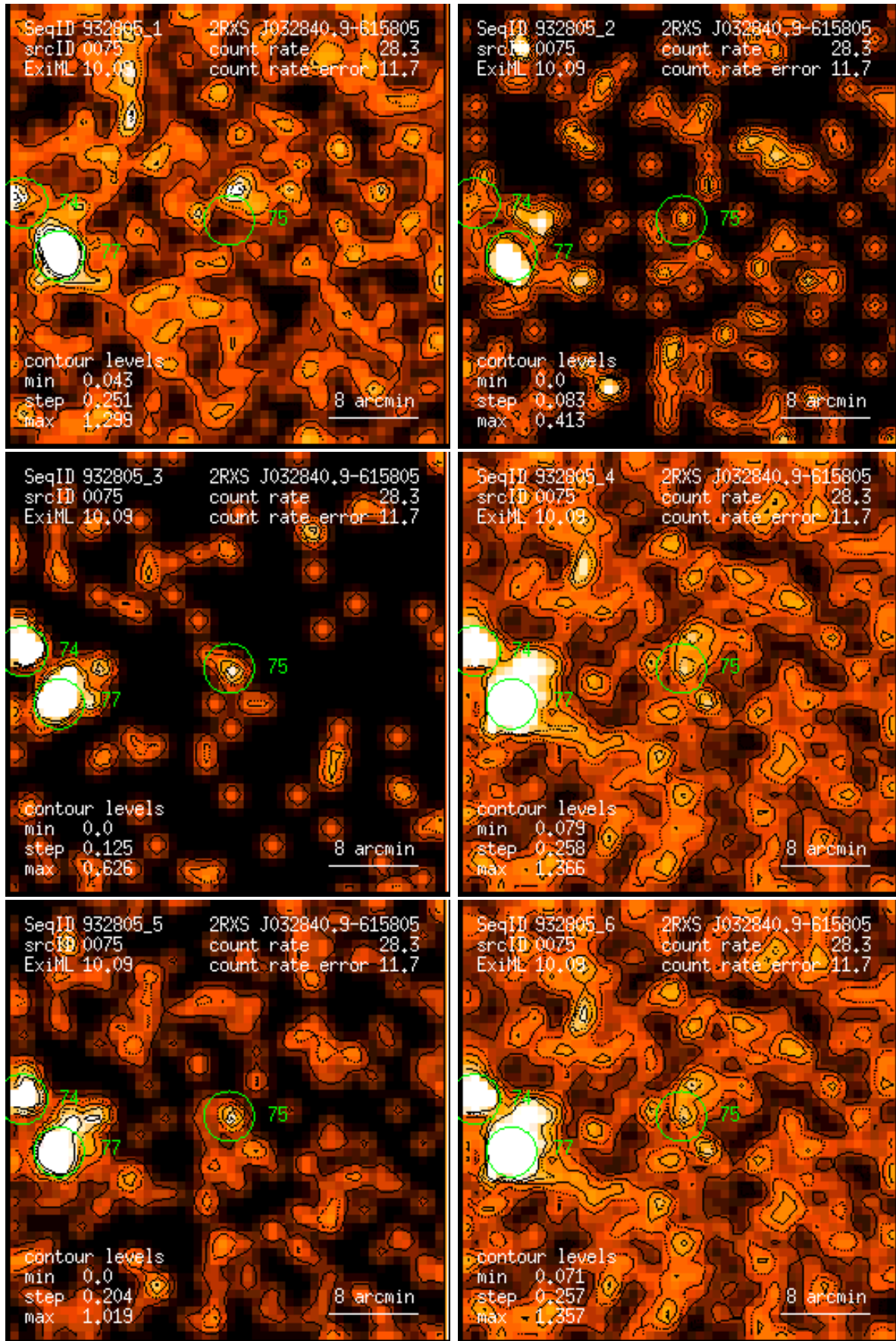
Figure 75: RASS 932805: detection 0075: band rate images, Gaussian filter: (1) PSPC channels 11 – 41, (2) 52 – 90, (3) 91 – 201, (4) 11 – 235, (5) 52 – 201, (6) 11 – 201. Broad band rates in counts/ks. Band rate contour levels in counts/ks/arcmin 2 .
