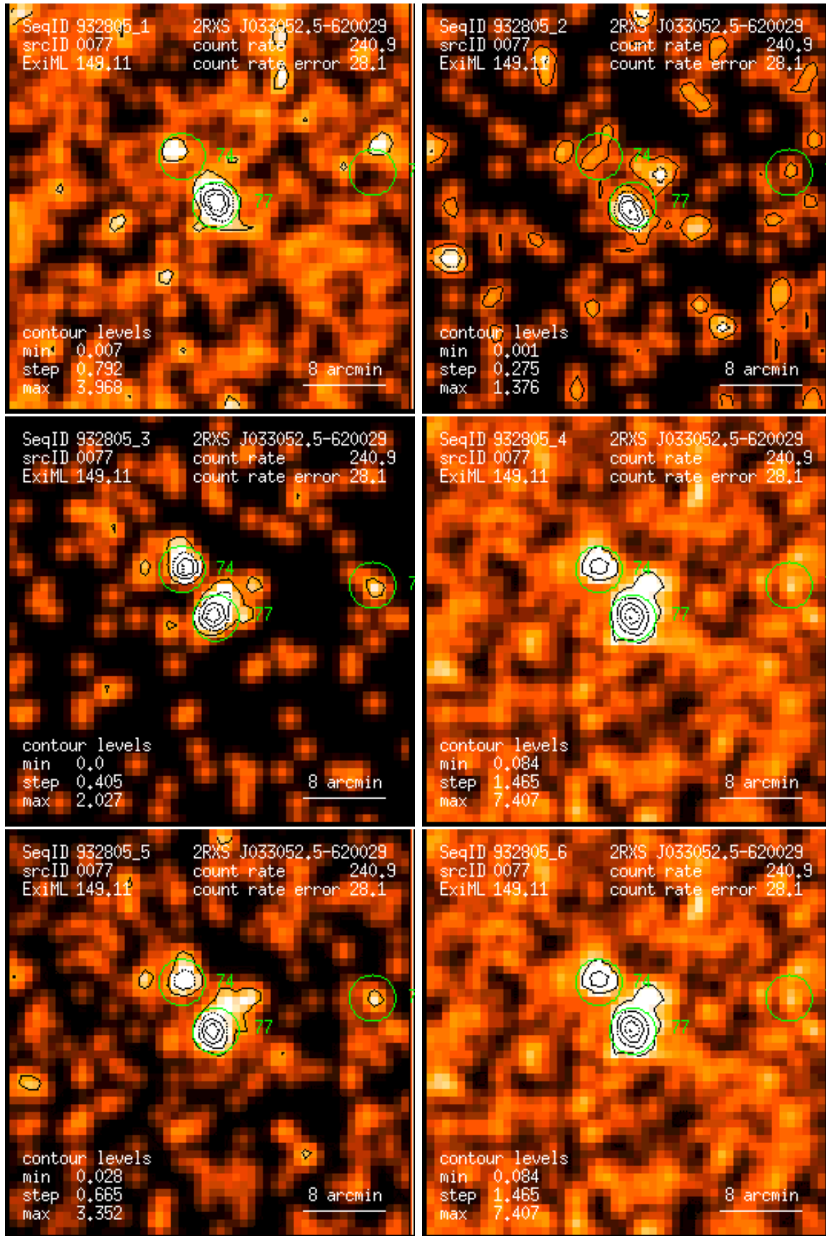
Figure 77: RASS 932805: detection 0077: band rate images, Gaussian filter: (1) PSPC channels 11 – 41, (2) 52 – 90, (3) 91 – 201, (4) 11 – 235, (5) 52 – 201, (6) 11 – 201. Broad band rates in counts/ks. Band rate contour levels in counts/ks/arcmin 2 .
