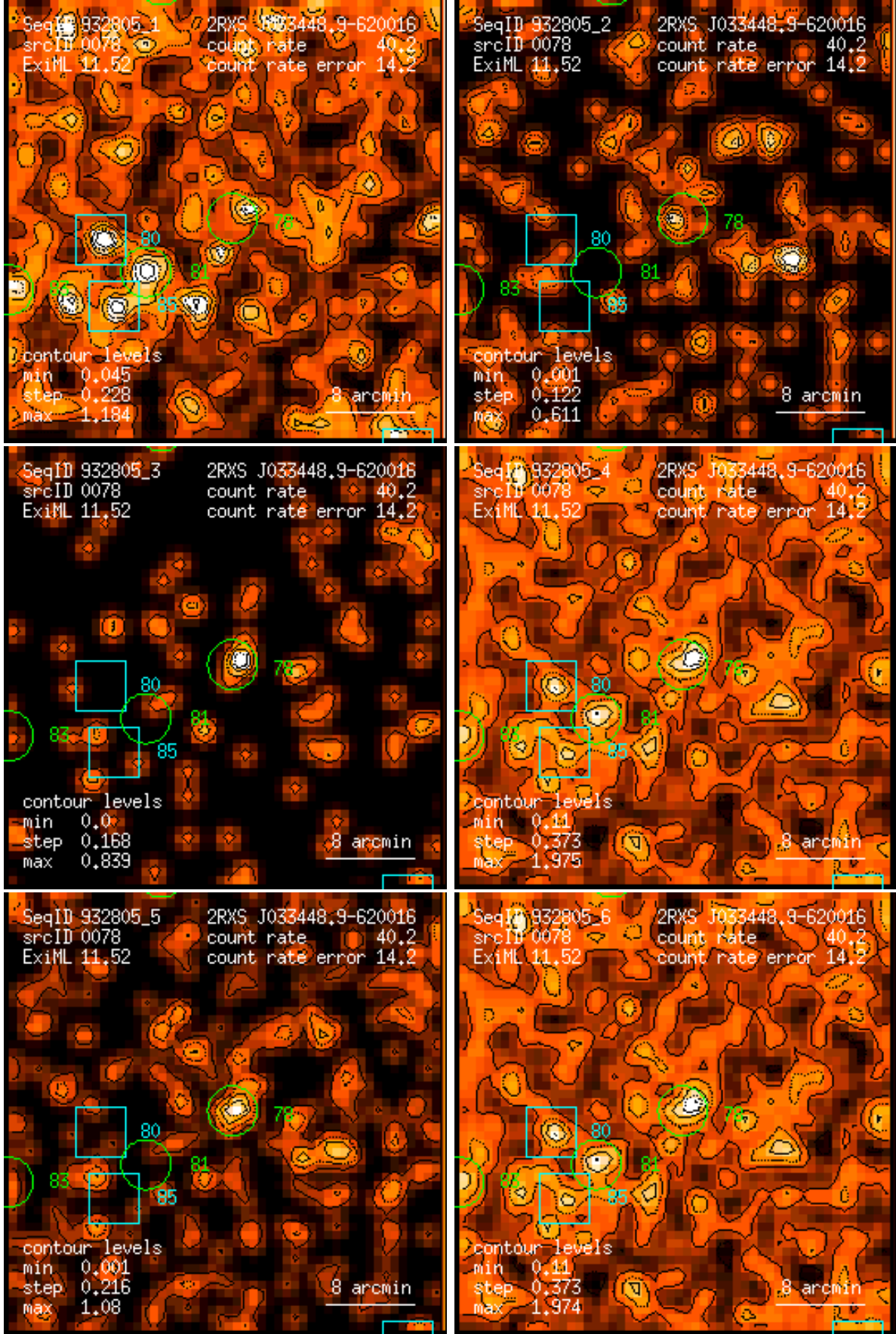
Figure 78: RASS 932805: detection 0078: band rate images, Gaussian filter: (1) PSPC channels 11 – 41, (2) 52 – 90, (3) 91 – 201, (4) 11 – 235, (5) 52 – 201, (6) 11 – 201. Broad band rates in counts/ks. Band rate contour levels in counts/ks/arcmin 2 .
