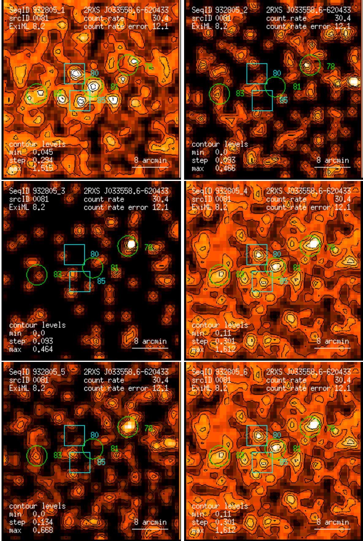
Figure 81: RASS 932805: detection 0081: band rate images, Gaussian filter: (1) PSPC channels 11 – 41, (2) 52 – 90, (3) 91 – 201, (4) 11 – 235, (5) 52 – 201, (6) 11 – 201. Broad band rates in counts/ks. Band rate contour levels in counts/ks/arcmin 2 .
