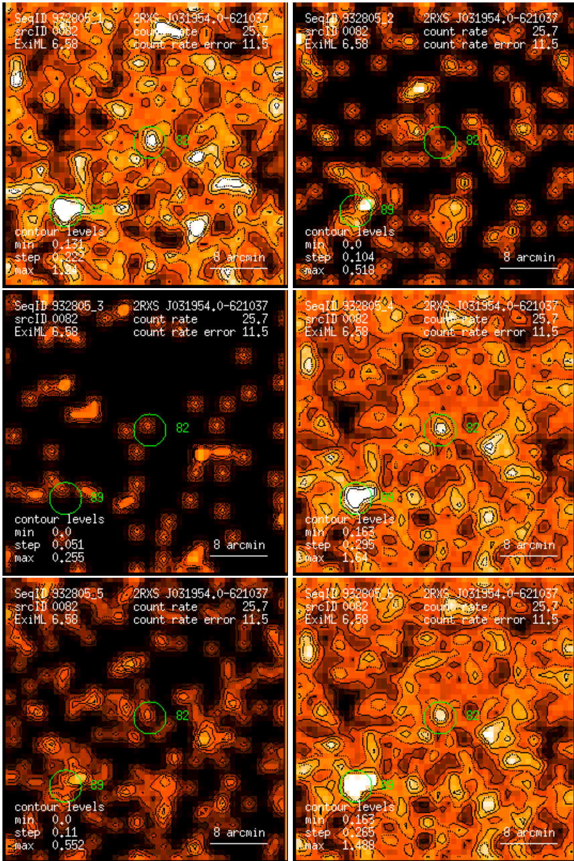
Figure 82: RASS 932805: detection 0082: band rate images, Gaussian filter: (1) PSPC channels 11 – 41, (2) 52 – 90, (3) 91 – 201, (4) 11 – 235, (5) 52 – 201, (6) 11 – 201. Broad band rates in counts/ks. Band rate contour levels in counts/ks/arcmin 2 .
