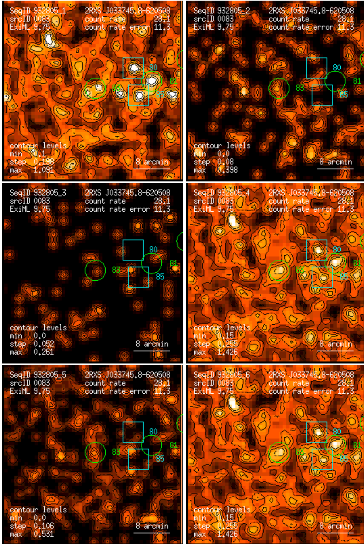
Figure 83: RASS 932805: detection 0083: band rate images, Gaussian filter: (1) PSPC channels 11 – 41, (2) 52 – 90, (3) 91 – 201, (4) 11 – 235, (5) 52 – 201, (6) 11 – 201. Broad band rates in counts/ks. Band rate contour levels in counts/ks/arcmin 2 .
