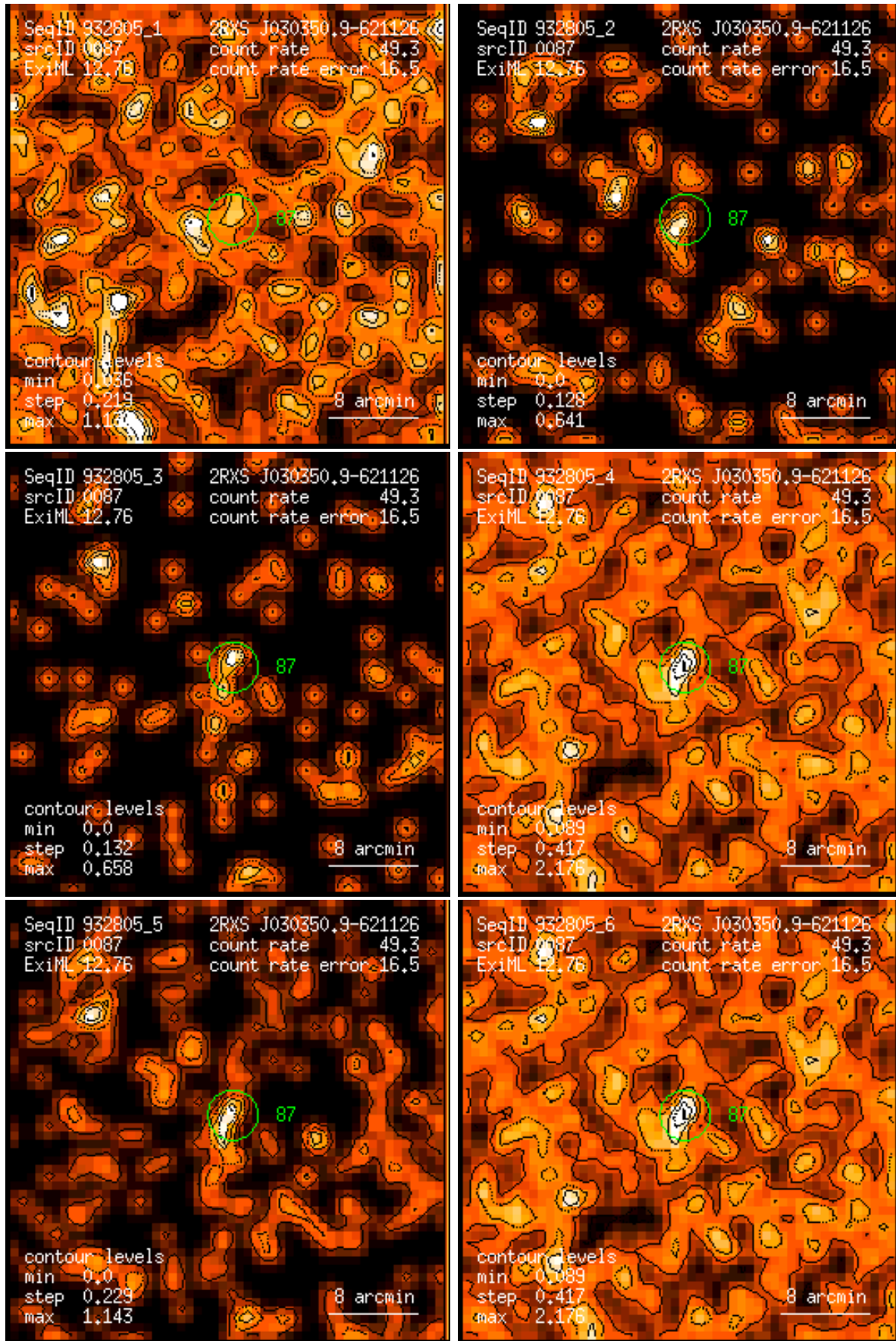
Figure 87: RASS 932805: detection 0087: band rate images, Gaussian filter: (1) PSPC channels 11 – 41, (2) 52 – 90, (3) 91 – 201, (4) 11 – 235, (5) 52 – 201, (6) 11 – 201. Broad band rates in counts/ks. Band rate contour levels in counts/ks/arcmin 2 .
