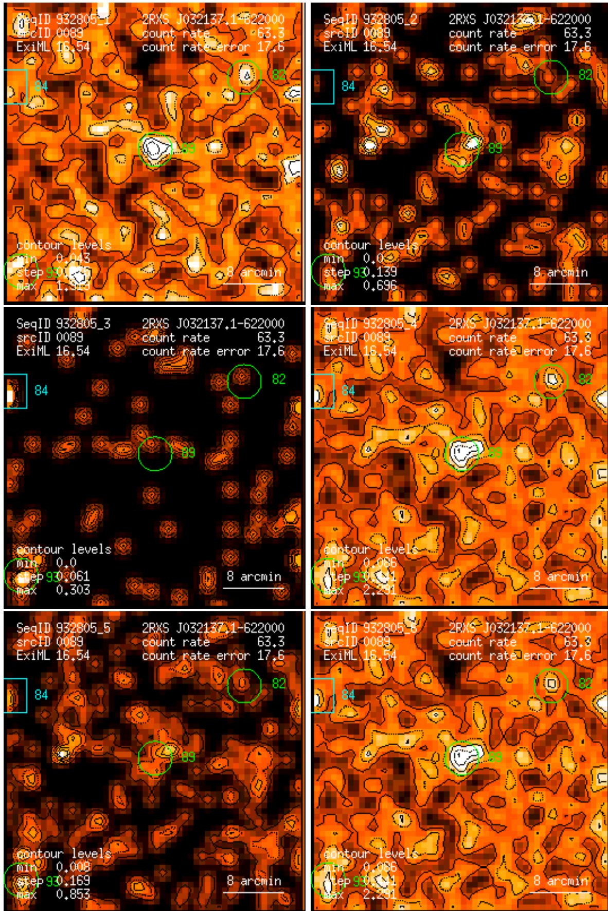
Figure 89: RASS 932805: detection 0089: band rate images, Gaussian filter: (1) PSPC channels 11 – 41, (2) 52 – 90, (3) 91 – 201, (4) 11 – 235, (5) 52 – 201, (6) 11 – 201. Broad band rates in counts/ks. Band rate contour levels in counts/ks/arcmin 2 .
