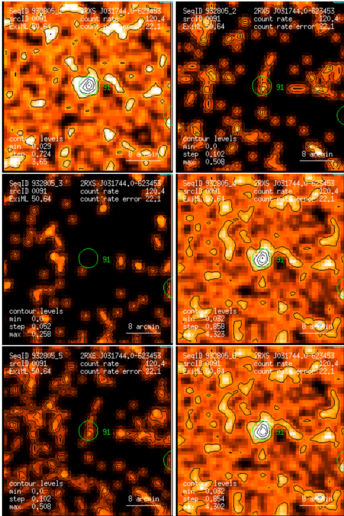
Figure 91: RASS 932805: detection 0091: band rate images, Gaussian filter: (1) PSPC channels 11 – 41, (2) 52 – 90, (3) 91 – 201, (4) 11 – 235, (5) 52 – 201, (6) 11 – 201. Broad band rates in counts/ks. Band rate contour levels in counts/ks/arcmin 2 .
