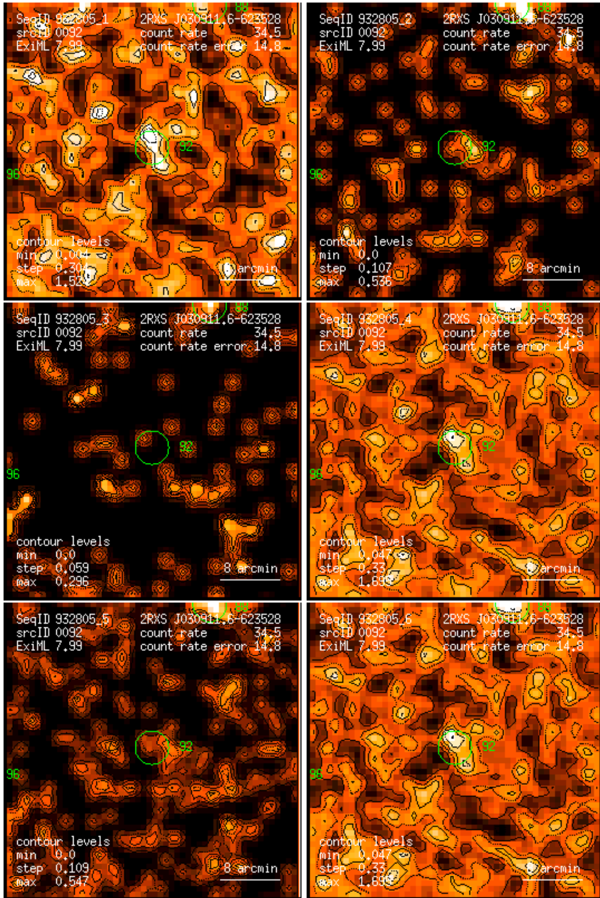
Figure 92: RASS 932805: detection 0092: band rate images, Gaussian filter: (1) PSPC channels 11 – 41, (2) 52 – 90, (3) 91 – 201, (4) 11 – 235, (5) 52 – 201, (6) 11 – 201. Broad band rates in counts/ks. Band rate contour levels in counts/ks/arcmin 2 .
