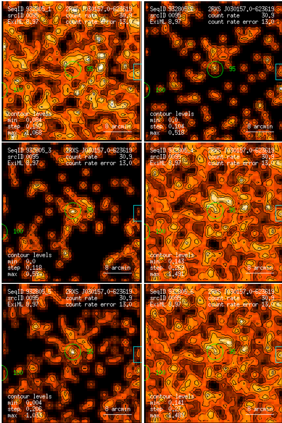
Figure 95: RASS 932805: detection 0095: band rate images, Gaussian filter: (1) PSPC channels 11 – 41, (2) 52 – 90, (3) 91 – 201, (4) 11 – 235, (5) 52 – 201, (6) 11 – 201. Broad band rates in counts/ks. Band rate contour levels in counts/ks/arcmin 2 .
