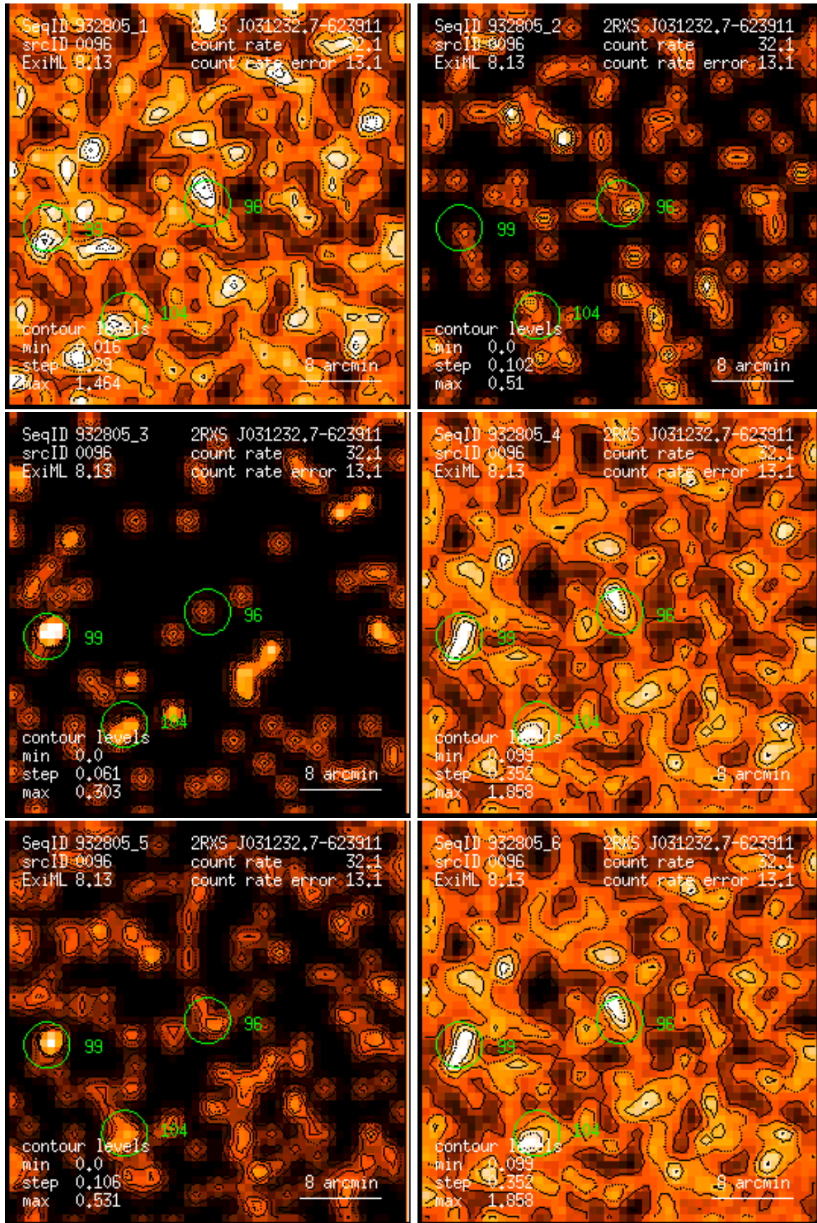
Figure 96: RASS 932805: detection 0096: band rate images, Gaussian filter: (1) PSPC channels 11 – 41, (2) 52 – 90, (3) 91 – 201, (4) 11 – 235, (5) 52 – 201, (6) 11 – 201. Broad band rates in counts/ks. Band rate contour levels in counts/ks/arcmin 2 .
