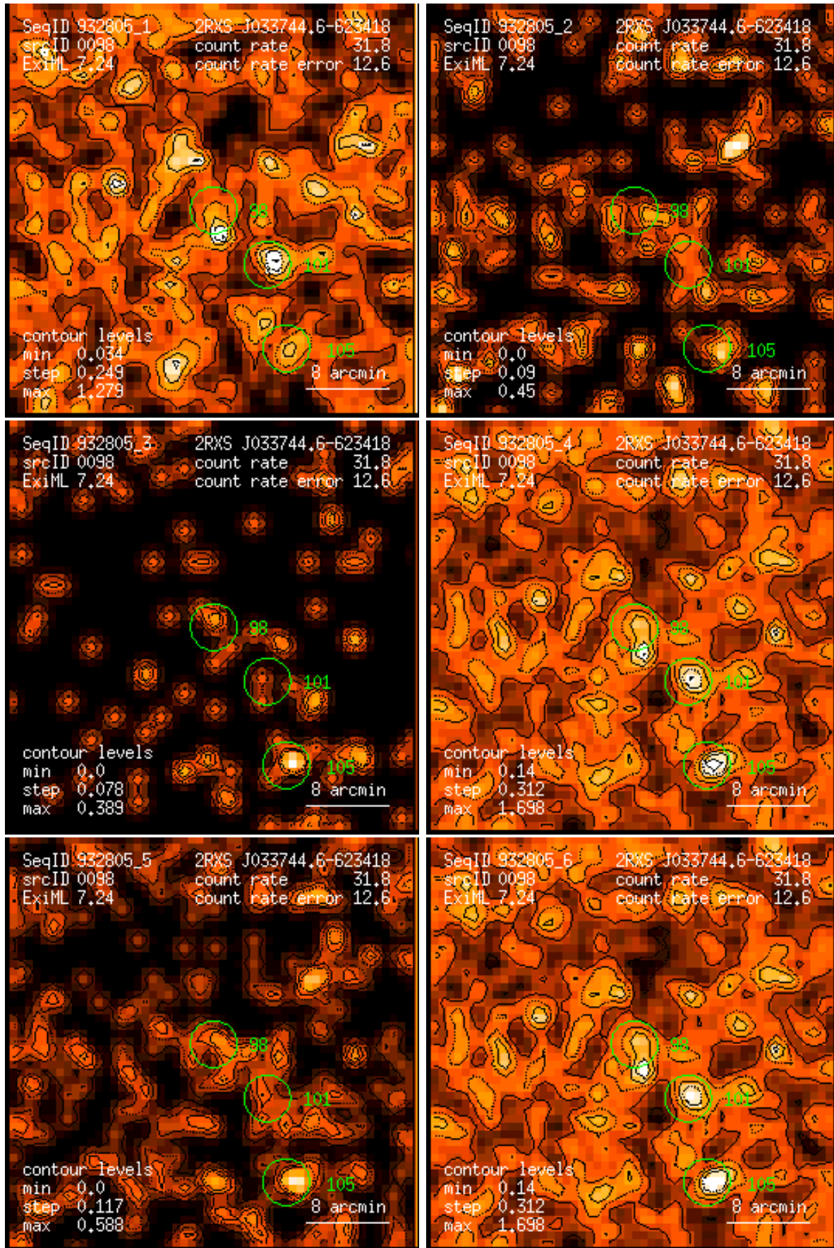
Figure 98: RASS 932805: detection 0098: band rate images, Gaussian filter: (1) PSPC channels 11 – 41, (2) 52 – 90, (3) 91 – 201, (4) 11 – 235, (5) 52 – 201, (6) 11 – 201. Broad band rates in counts/ks. Band rate contour levels in counts/ks/arcmin 2 .
