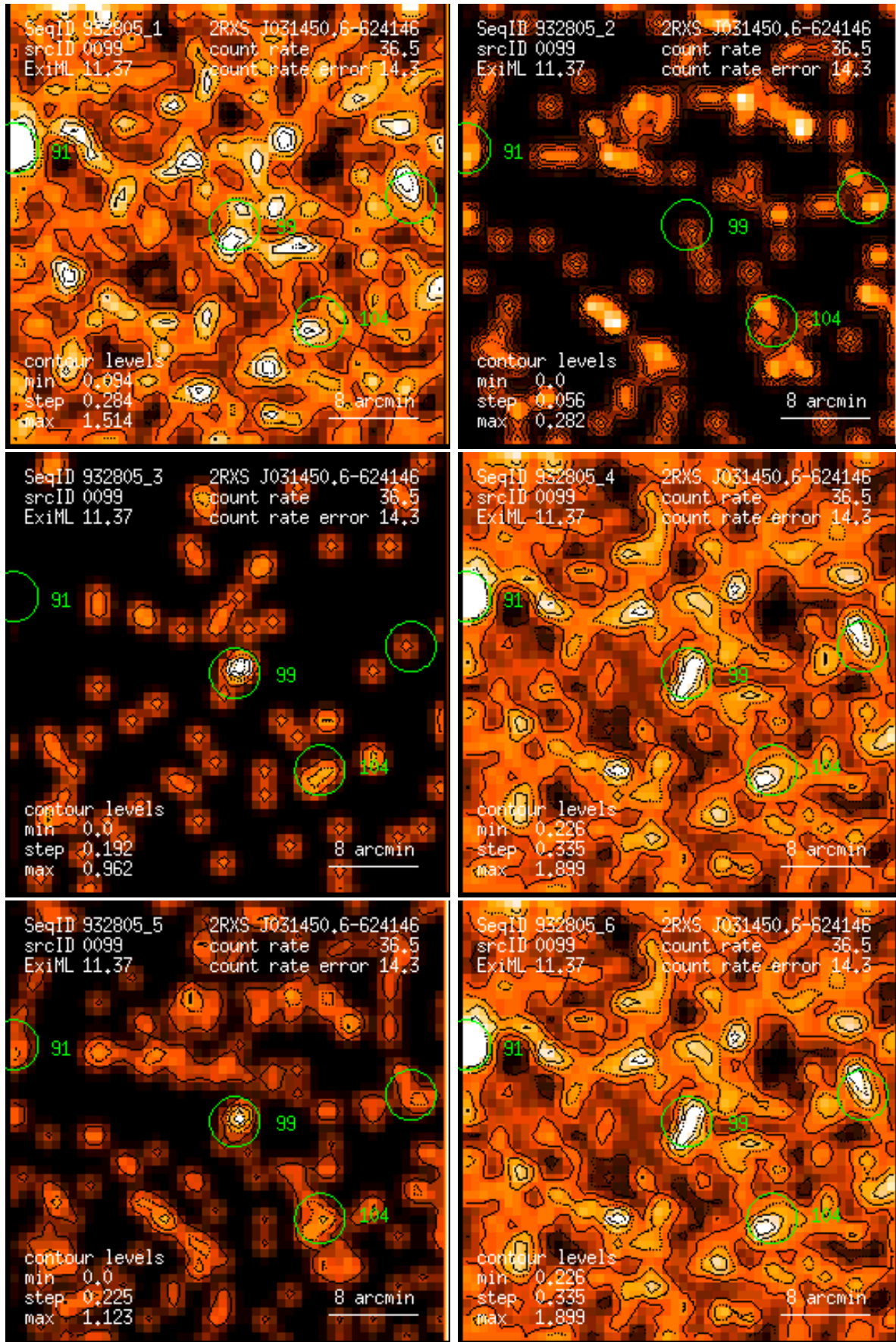
Figure 99: RASS 932805: detection 0099: band rate images, Gaussian filter: (1) PSPC channels 11 – 41, (2) 52 – 90, (3) 91 – 201, (4) 11 – 235, (5) 52 – 201, (6) 11 – 201. Broad band rates in counts/ks. Band rate contour levels in counts/ks/arcmin 2 .
