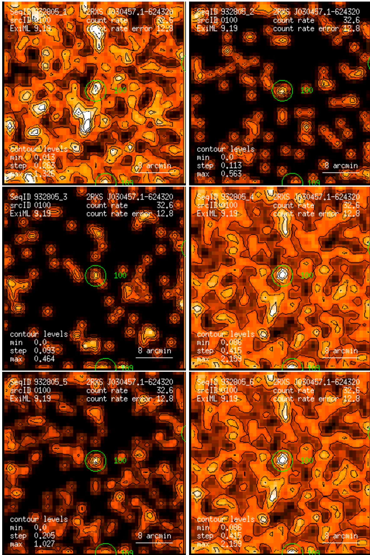
Figure 100: RASS 932805: detection 0100: band rate images, Gaussian filter: (1) PSPC channels 11 – 41, (2) 52 – 90, (3) 91 – 201, (4) 11 – 235, (5) 52 – 201, (6) 11 – 201. Broad band rates in counts/ks. Band rate contour levels in counts/ks/arcmin 2 .
