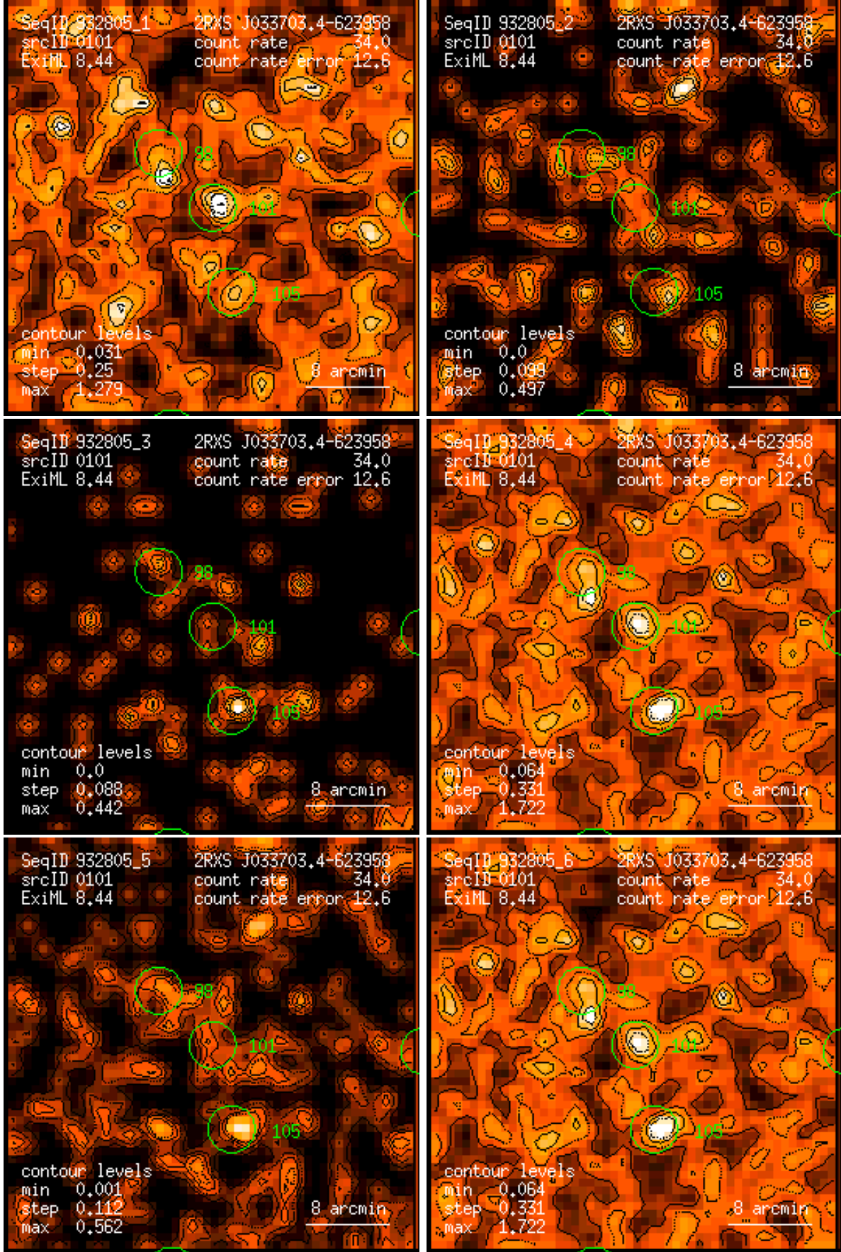
Figure 101: RASS 932805: detection 0101: band rate images, Gaussian filter: (1) PSPPC channels 11 – 41, (2) 52 – 90, (3) 91 – 201, (4) 11 – 235, (5) 52 – 201, (6) 11 – 201. Broad band rates in counts/ks. Band rate contour levels in counts/ks/arcmin 2 .
