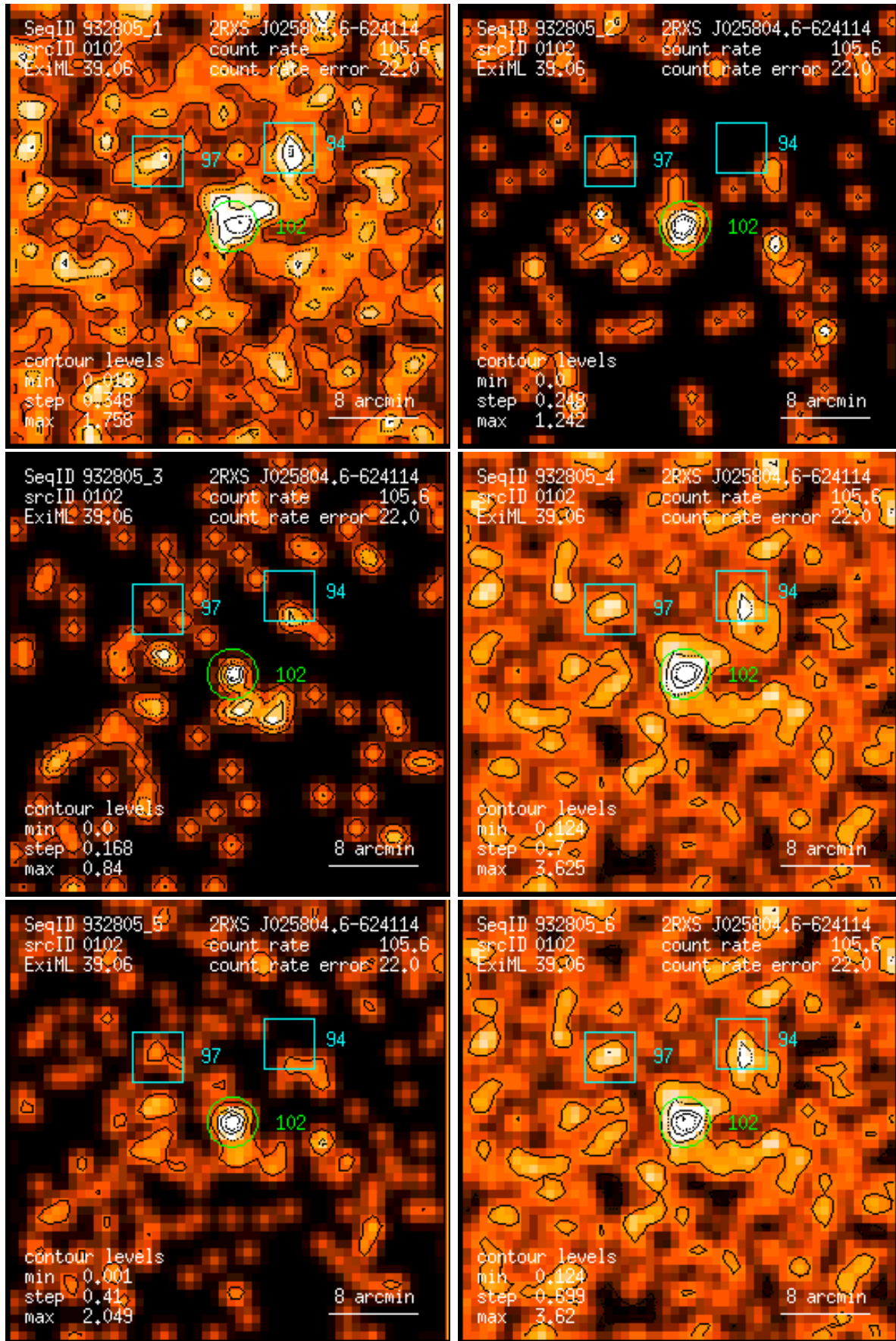
Figure 102: RASS 932805: detection 0102: band rate images, Gaussian filter: (1) PSPC channels 11 – 41, (2) 52 – 90, (3) 91 – 201, (4) 11 – 235, (5) 52 – 201, (6) 11 – 201. Broad band rates in counts/ks. Band rate contour levels in counts/ks/arcmin 2 .
