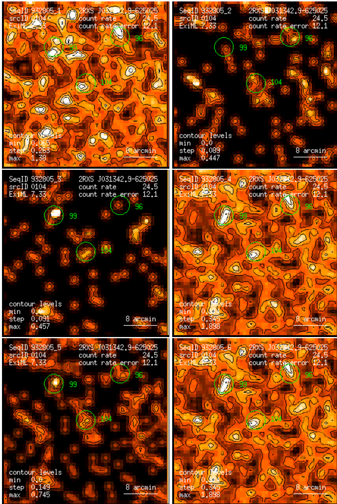
Figure 104: RASS 932805: detection 0104: band rate images, Gaussian filter: (1) PSPC channels 11 – 41, (2) 52 – 90, (3) 91 – 201, (4) 11 – 235, (5) 52 – 201, (6) 11 – 201. Broad band rates in counts/ks. Band rate contour levels in counts/ks/arcmin 2 .
