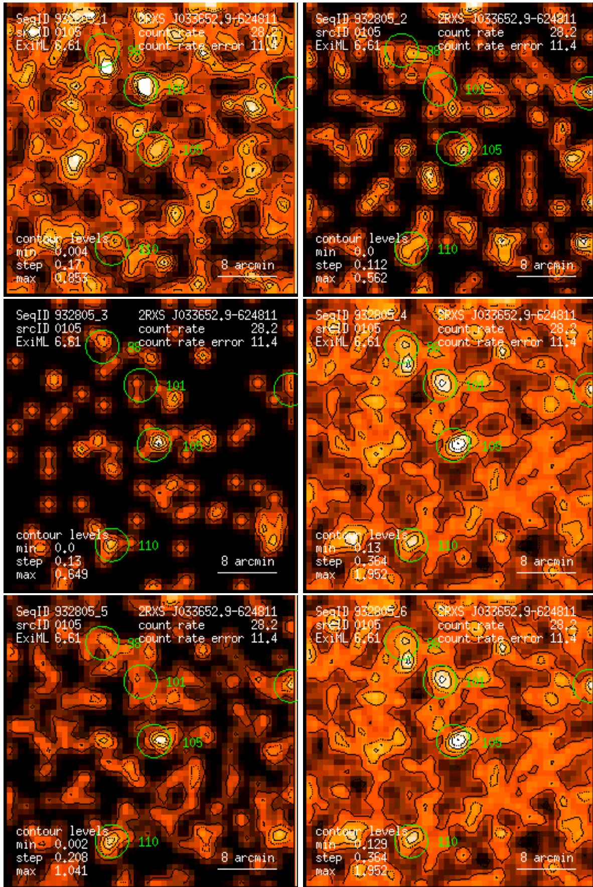
Figure 105: RASS 932805: detection 0105: band rate images, Gaussian filter: (1) PSPC channels 11 – 41, (2) 52 – 90, (3) 91 – 201, (4) 11 – 235, (5) 52 – 201, (6) 11 – 201. Broad band rates in counts/ks. Band rate contour levels in counts/ks/arcmin 2 .
