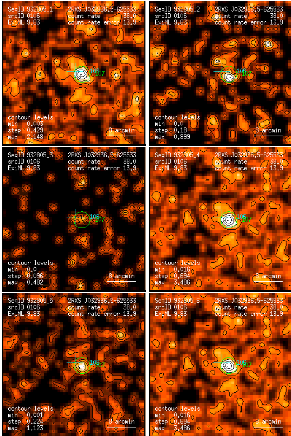
Figure 106: RASS 932805: detection 0106: band rate images, Gaussian filter: (1) PSPC channels 11 – 41, (2) 52 – 90, (3) 91 – 201, (4) 11 – 235, (5) 52 – 201, (6) 11 – 201. Broad band rates in counts/ks. Band rate contour levels in counts/ks/arcmin 2 .
