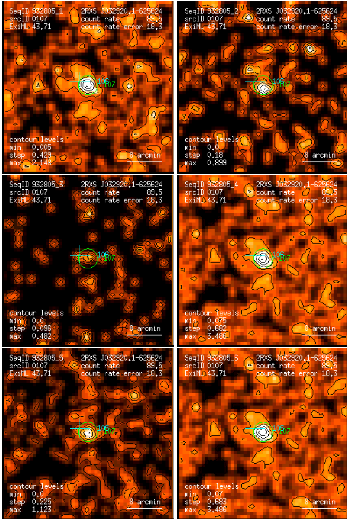
Figure 107: RASS 932805: detection 0107: band rate images, Gaussian filter: (1) PSPC channels 11 – 41, (2) 52 – 90, (3) 91 – 201, (4) 11 – 235, (5) 52 – 201, (6) 11 – 201. Broad band rates in counts/ks. Band rate contour levels in counts/ks/arcmin 2 .
