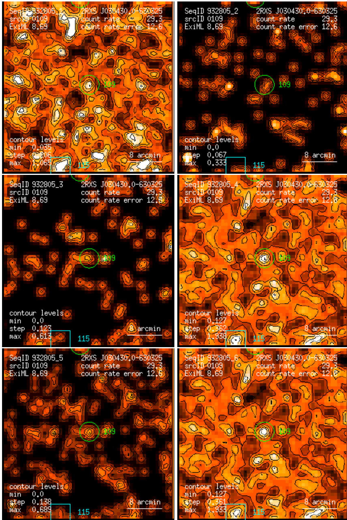
Figure 109: RASS 932805: detection 0109: band rate images, Gaussian filter: (1) PSPC channels 11 – 41, (2) 52 – 90, (3) 91 – 201, (4) 11 – 235, (5) 52 – 201, (6) 11 – 201. Broad band rates in counts/ks. Band rate contour levels in counts/ks/arcmin 2 .
