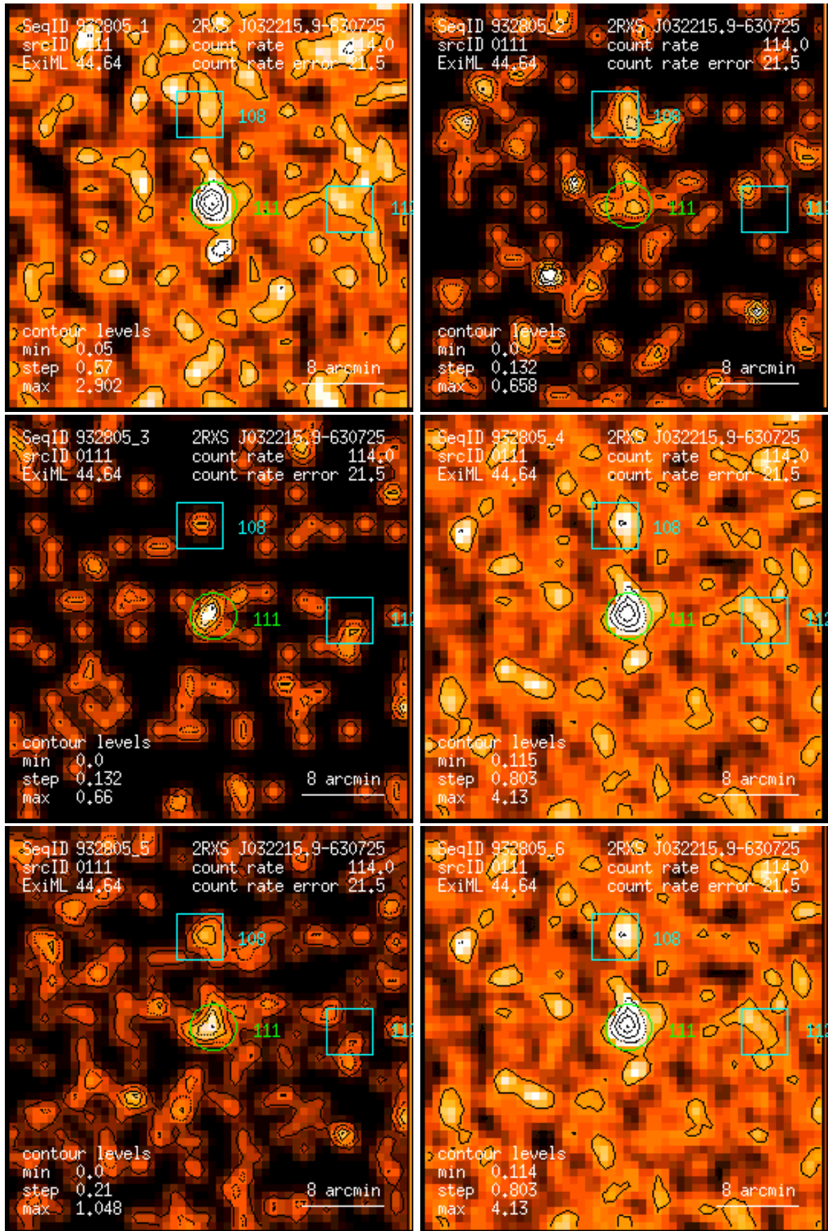
Figure 111: RASS 932805: detection 0111: band rate images, Gaussian filter: (1) PSPC channels 11 – 41, (2) 52 – 90, (3) 91 – 201, (4) 11 – 235, (5) 52 – 201, (6) 11 – 201. Broad band rates in counts/ks. Band rate contour levels in counts/ks/arcmin 2 .
