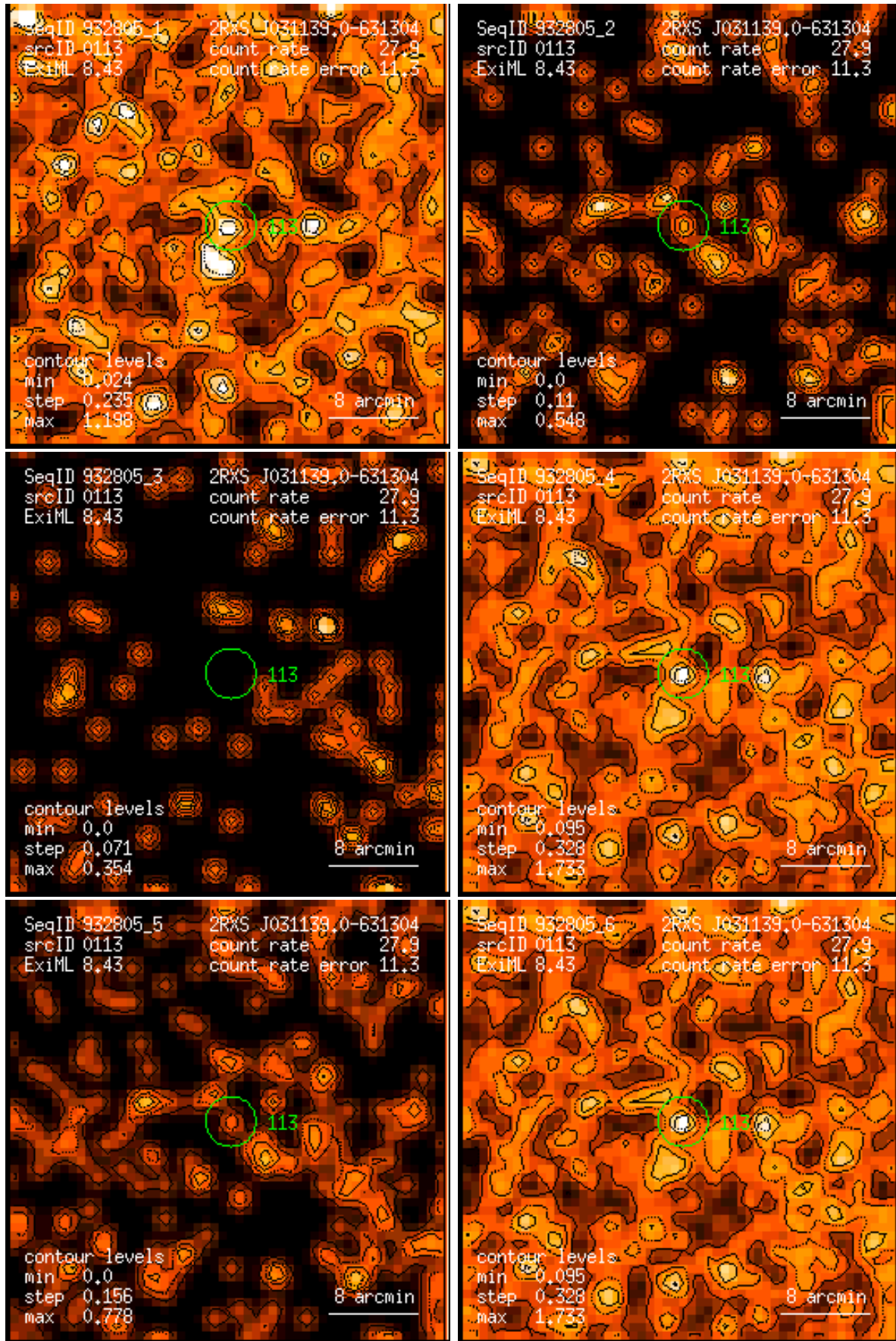
Figure 113: RASS 932805: detection 0113: band rate images, Gaussian filter: (1) PSPC channels 11 – 41, (2) 52 – 90, (3) 91 – 201, (4) 11 – 235, (5) 52 – 201, (6) 11 – 201. Broad band rates in counts/ks. Band rate contour levels in counts/ks/arcmin 2 .
