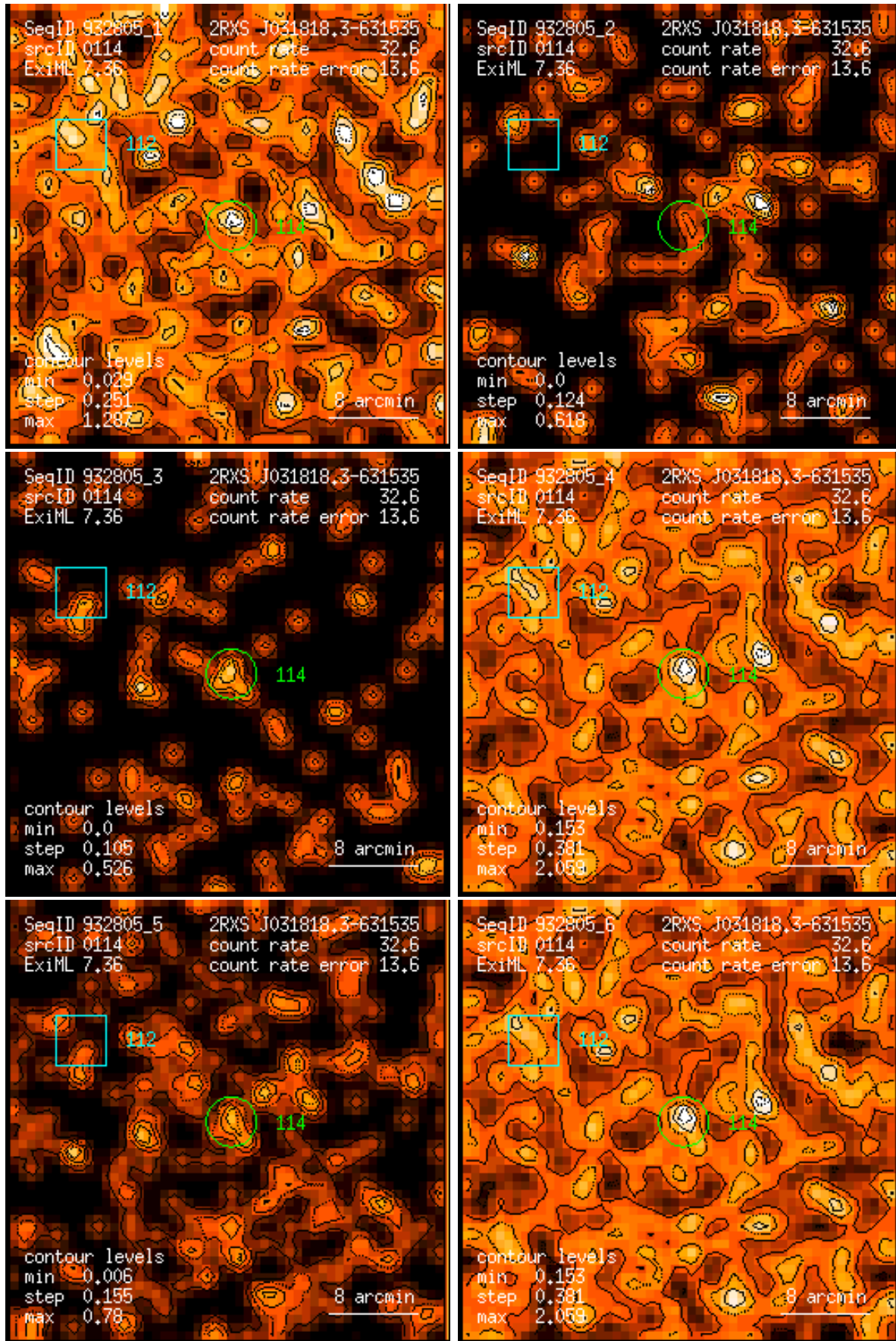
Figure 114: RASS 932805: detection 0114: band rate images, Gaussian filter: (1) PSPC channels 11 – 41, (2) 52 – 90, (3) 91 – 201, (4) 11 – 235, (5) 52 – 201, (6) 11 – 201. Broad band rates in counts/ks. Band rate contour levels in counts/ks/arcmin 2 .
