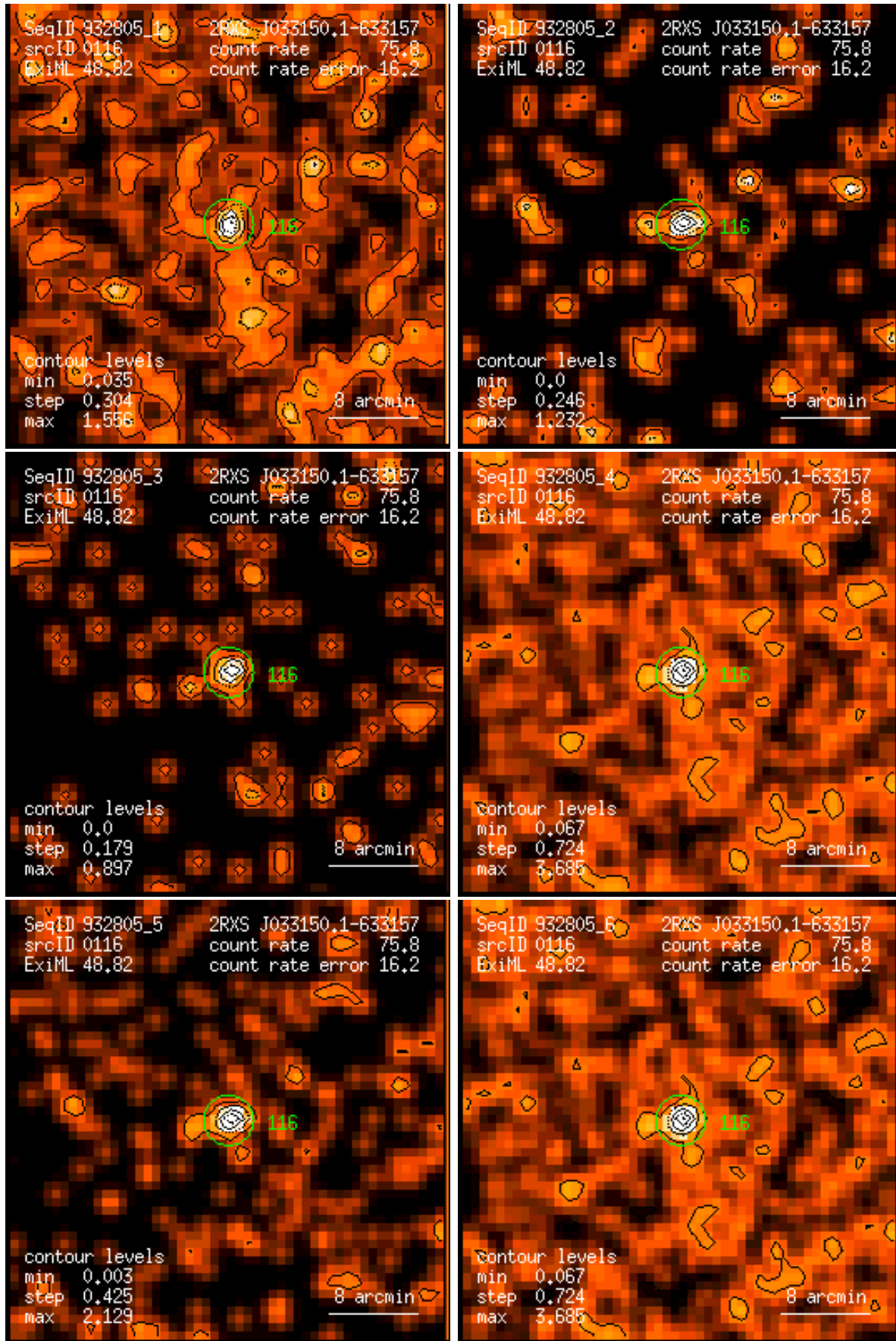
Figure 116: RASS 932805: detection 0116: band rate images, Gaussian filter: (1) PSPC channels 11 – 41, (2) 52 – 90, (3) 91 – 201, (4) 11 – 235, (5) 52 – 201, (6) 11 – 201. Broad band rates in counts/ks. Band rate contour levels in counts/ks/arcmin 2 .
