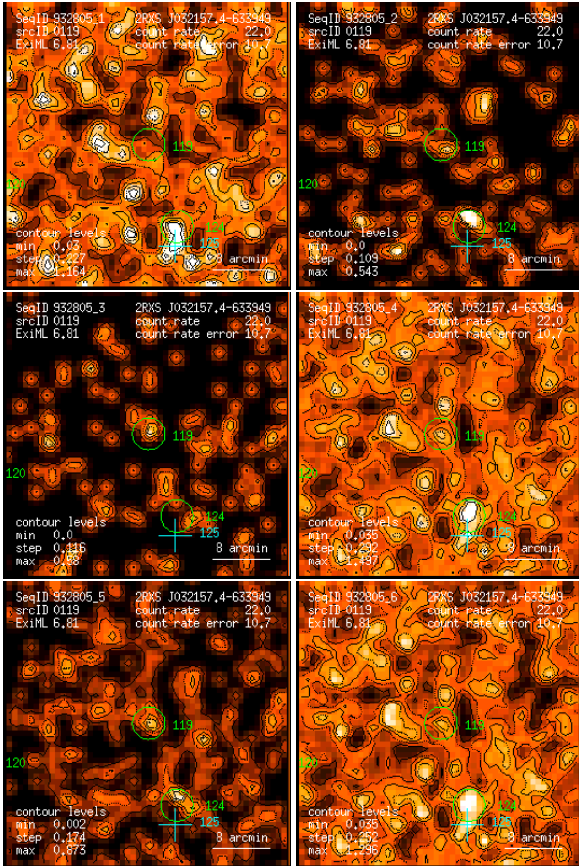
Figure 119: RASS 932805: detection 0119: band rate images, Gaussian filter: (1) PSPC channels 11 – 41, (2) 52 – 90, (3) 91 – 201, (4) 11 – 235, (5) 52 – 201, (6) 11 – 201. Broad band rates in counts/ks. Band rate contour levels in counts/ks/arcmin 2 .
