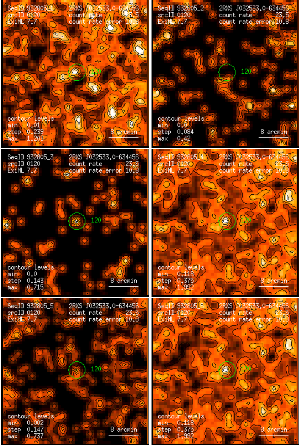
Figure 120: RASS 932805: detection 0120: band rate images, Gaussian filter: (1) PSPC channels 11 – 41, (2) 52 – 90, (3) 91 – 201, (4) 11 – 235, (5) 52 – 201, (6) 11 – 201. Broad band rates in counts/ks. Band rate contour levels in counts/ks/arcmin 2 .
