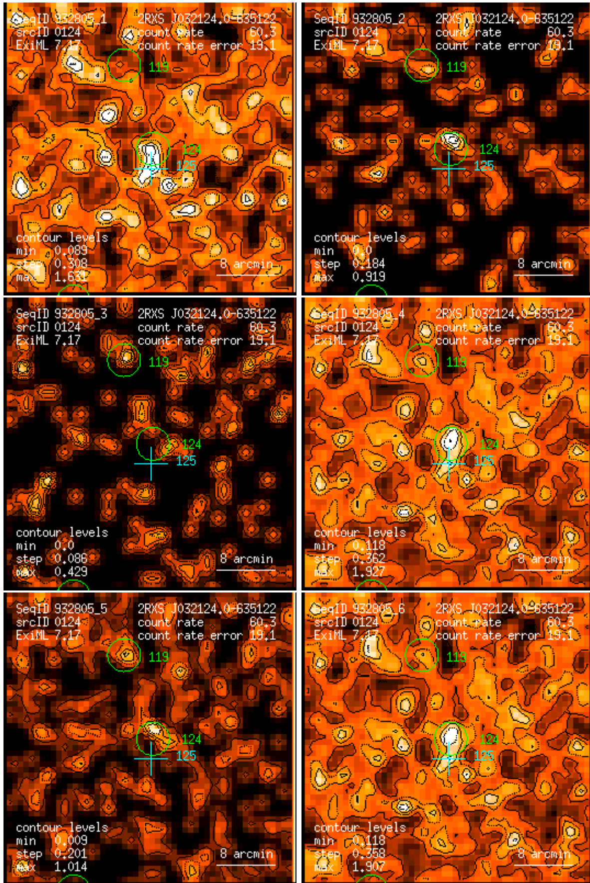
Figure 124: RASS 932805: detection 0124: band rate images, Gaussian filter: (1) PSPC channels 11 – 41, (2) 52 – 90, (3) 91 – 201, (4) 11 – 235, (5) 52 – 201, (6) 11 – 201. Broad band rates in counts/ks. Band rate contour levels in counts/ks/arcmin 2 .
